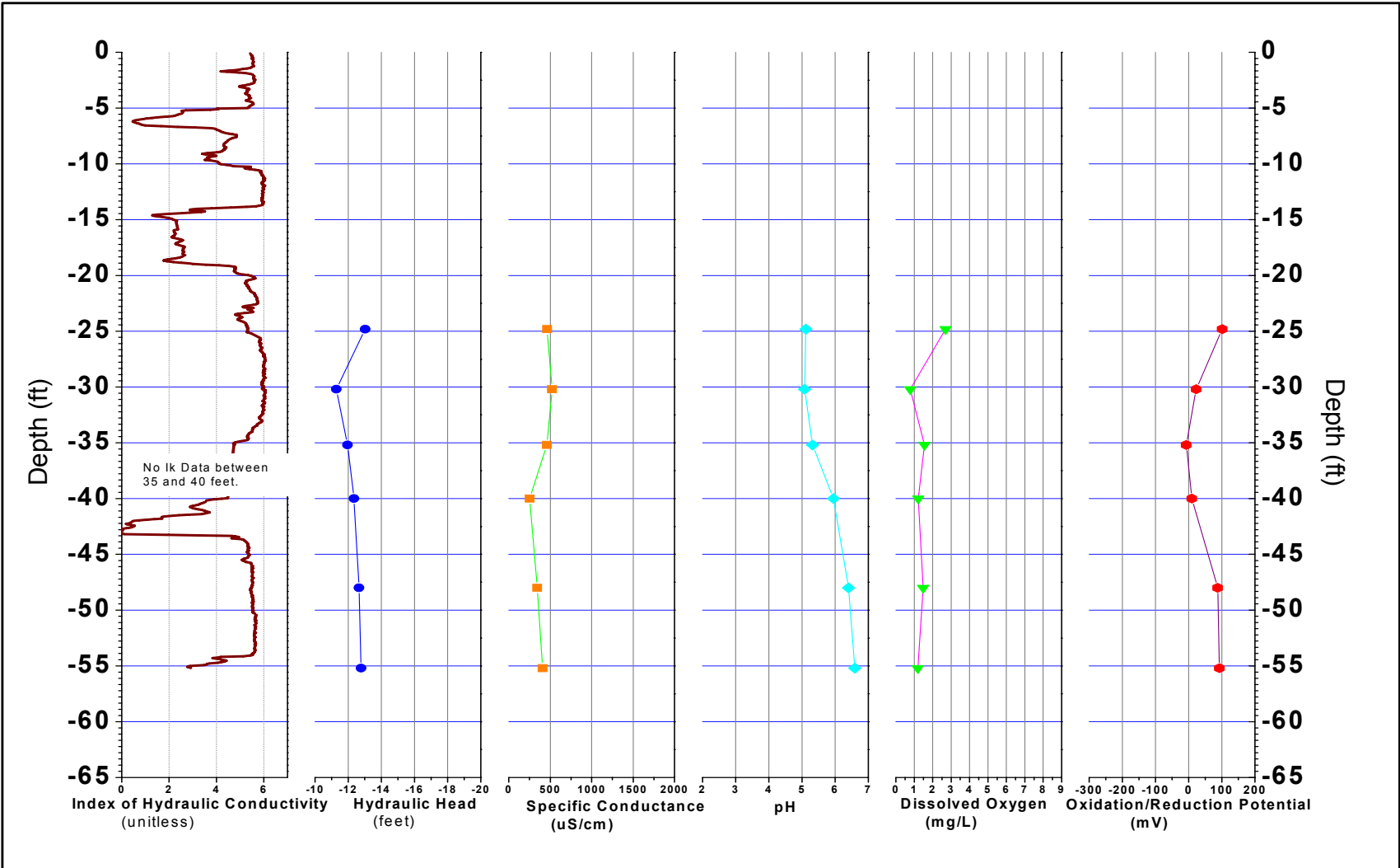
FIGURE B-225, I_k RECORD AND PHYSICO-CHEMICAL PARAMETERS ERM, Wayland, Massachusetts
