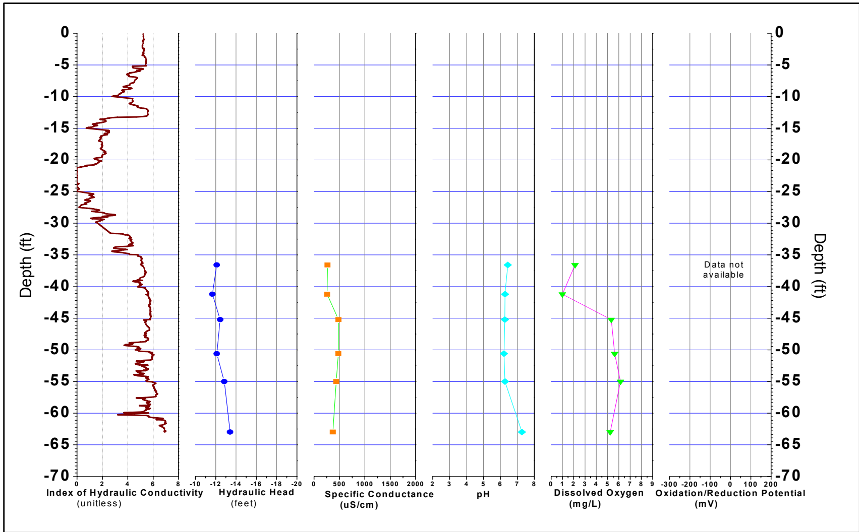
FIGURE B-240, I_k RECORD AND PHYSICO-CHEMICAL PARAMETERS ERM, Wayland, Massachusetts
