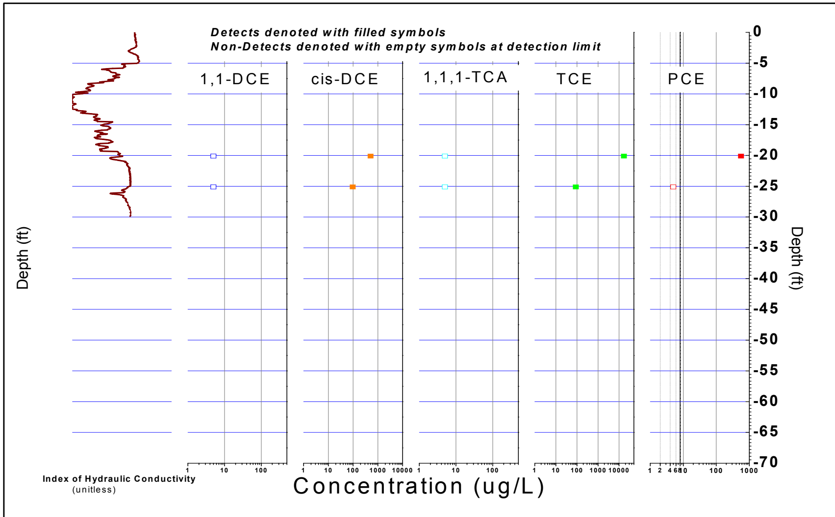
FIGURE B-241, I_K RECORD AND SELECTED VOC ANALYTICAL RESULTS ERM, Wayland, Massachusetts
