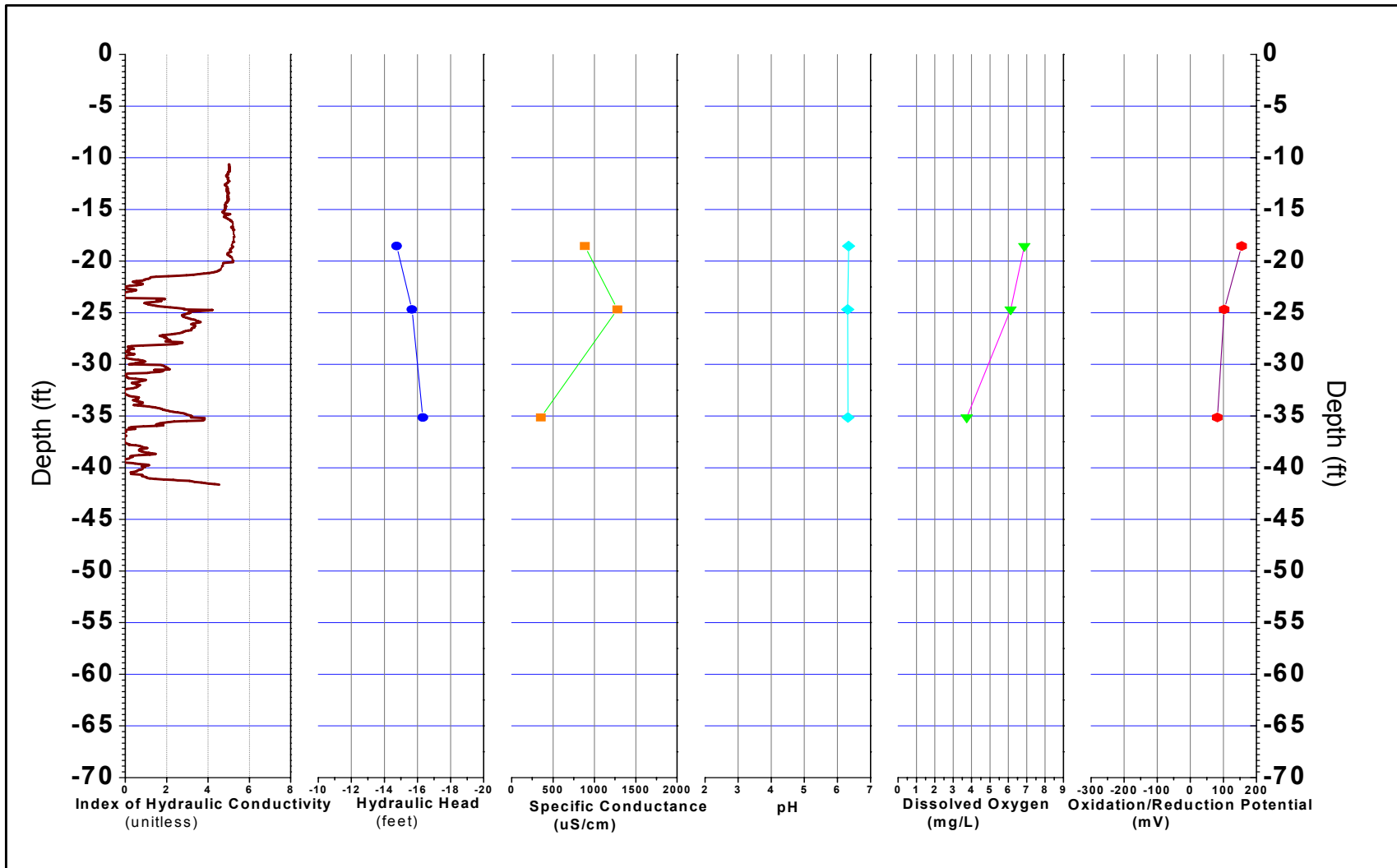
FIGURE B-201, I k RECORD AND PHYSICO-CHEMICAL PARAMETERS ERM, Wayland, Massachusetts
