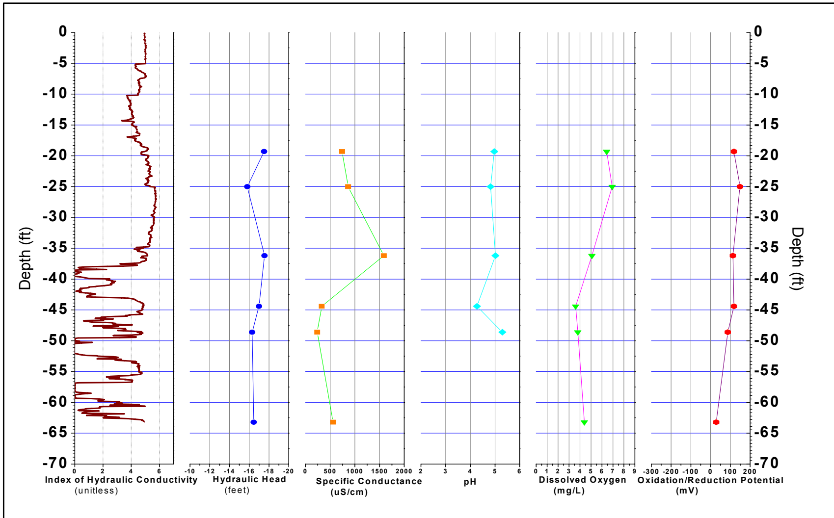
FIGURE B-204, I k RECORD AND PHYSICO-CHEMICAL PARAMETERS ERM, Wayland, Massachusetts
