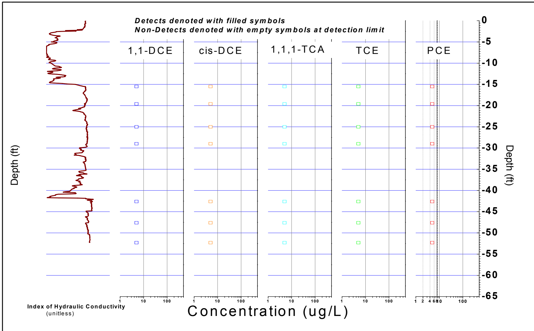
FIGURE B-234, I_k RECORD AND SELECTED VOC ANALYTICAL RESULTS ERM, Wayland, Massachusetts
