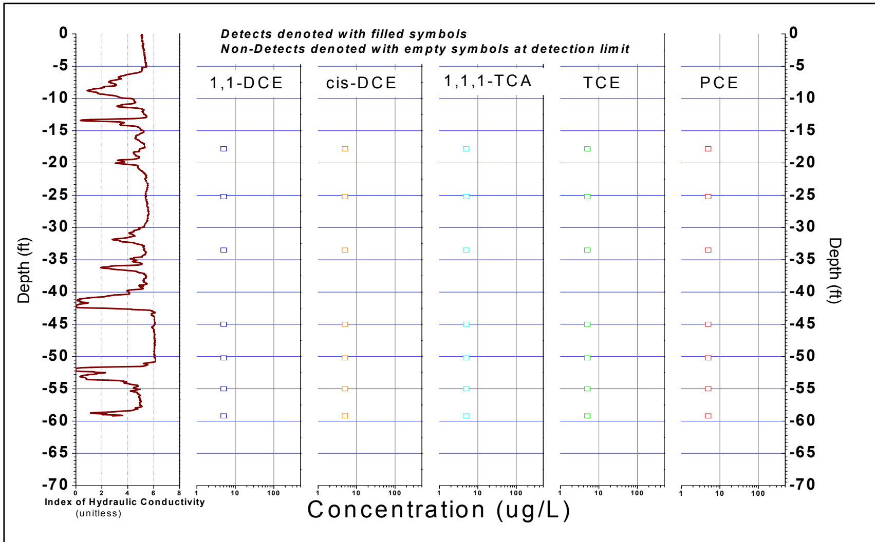
FIGURE B-233, I_k RECORD AND SELECTED VOC ANALYTICAL RESULTS ERM, Wayland, Massachusetts
