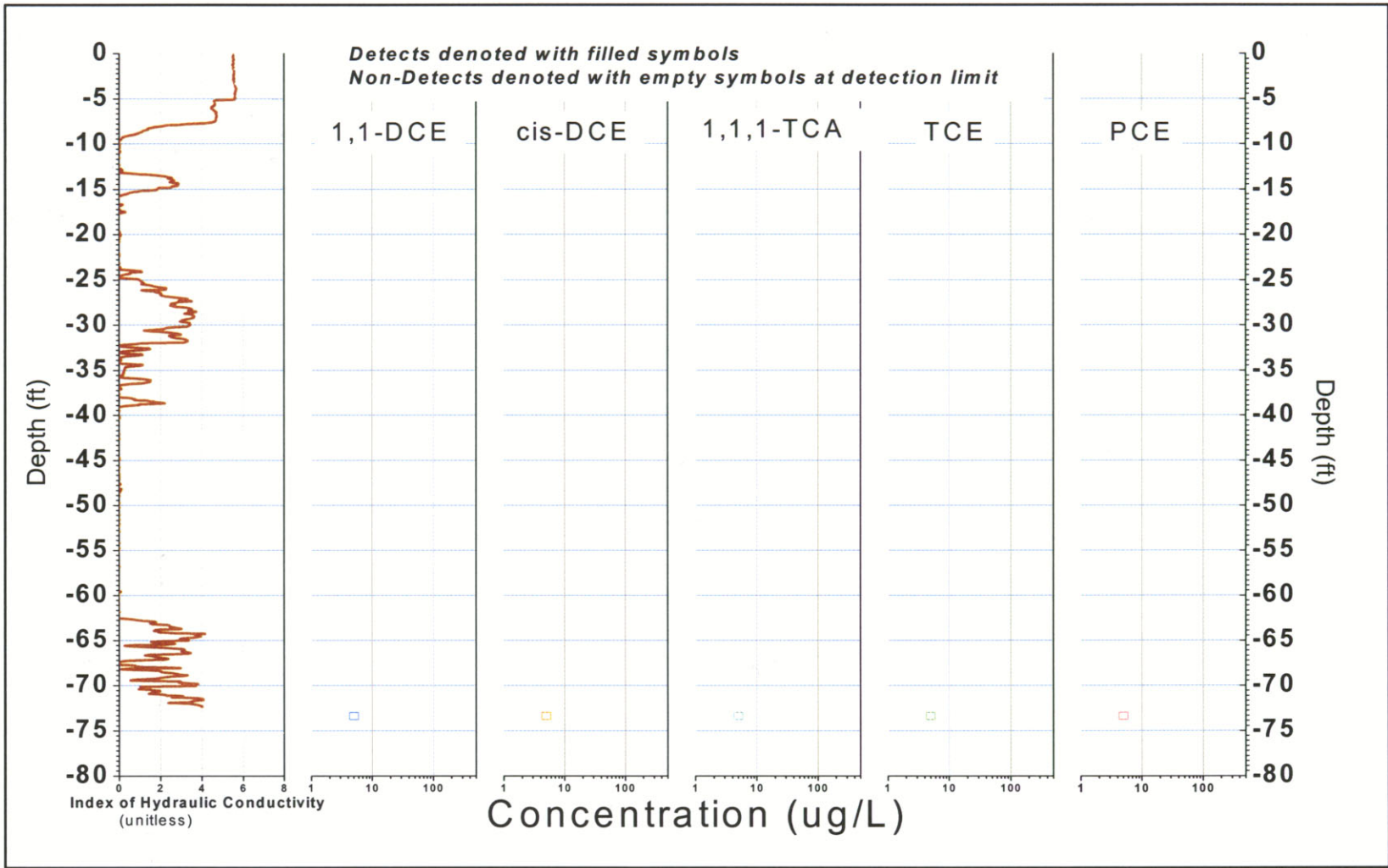
FIGURE B-239, I k RECORD AND SELECTED VOC ANALYTICAL RESULTS ERM, Wayland, Massachusetts
