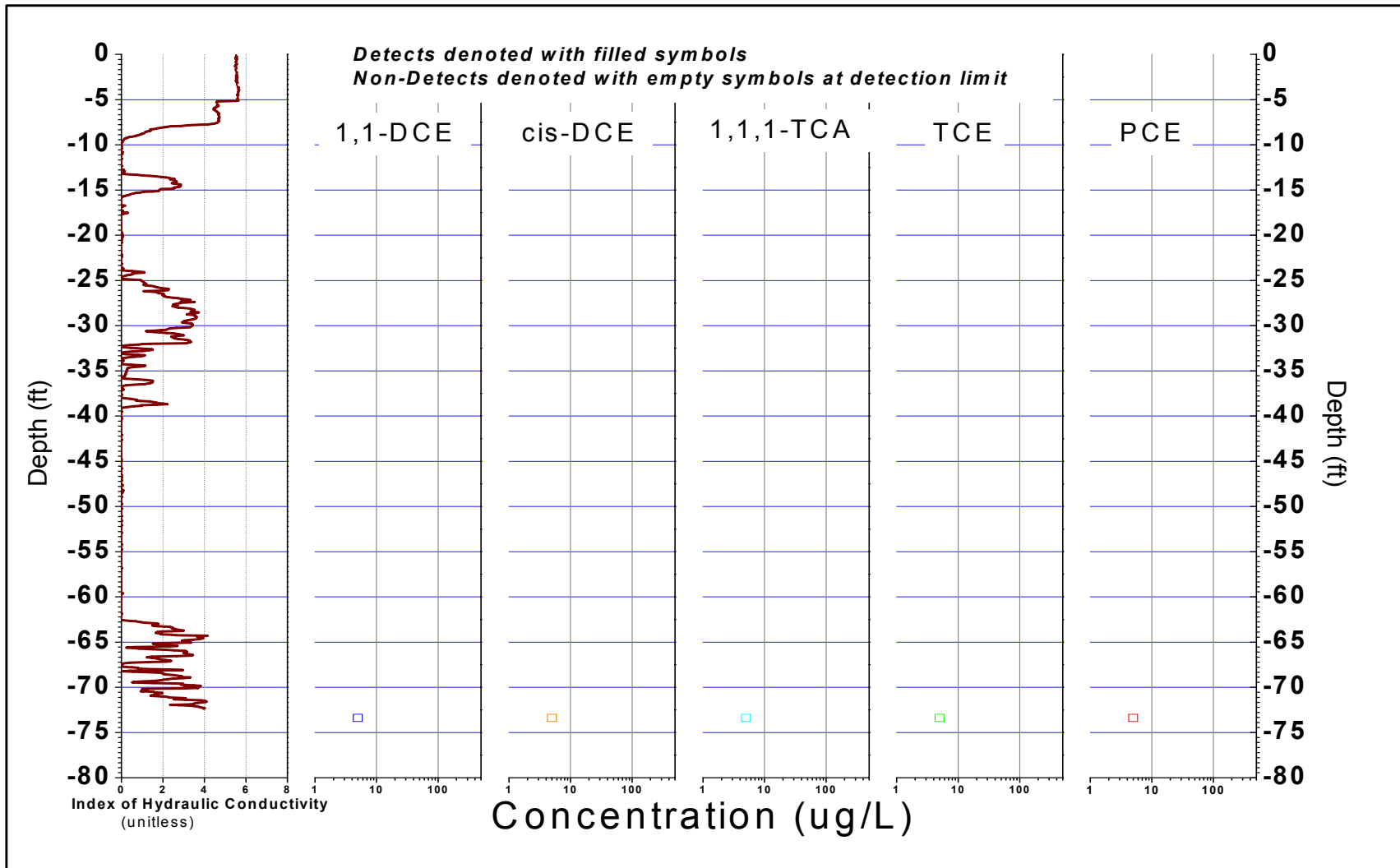
FIGURE B-239, I k RECORD AND SELECTED VOC ANALYTICAL RESULTS ERM, Wayland, Massachusetts
