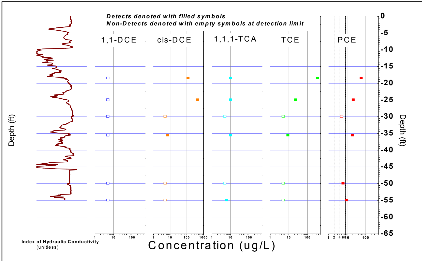
FIGURE B-228, I_k RECORD AND SELECTED VOC ANALYTICAL RESULTS ERM, Wayland, Massachusetts
