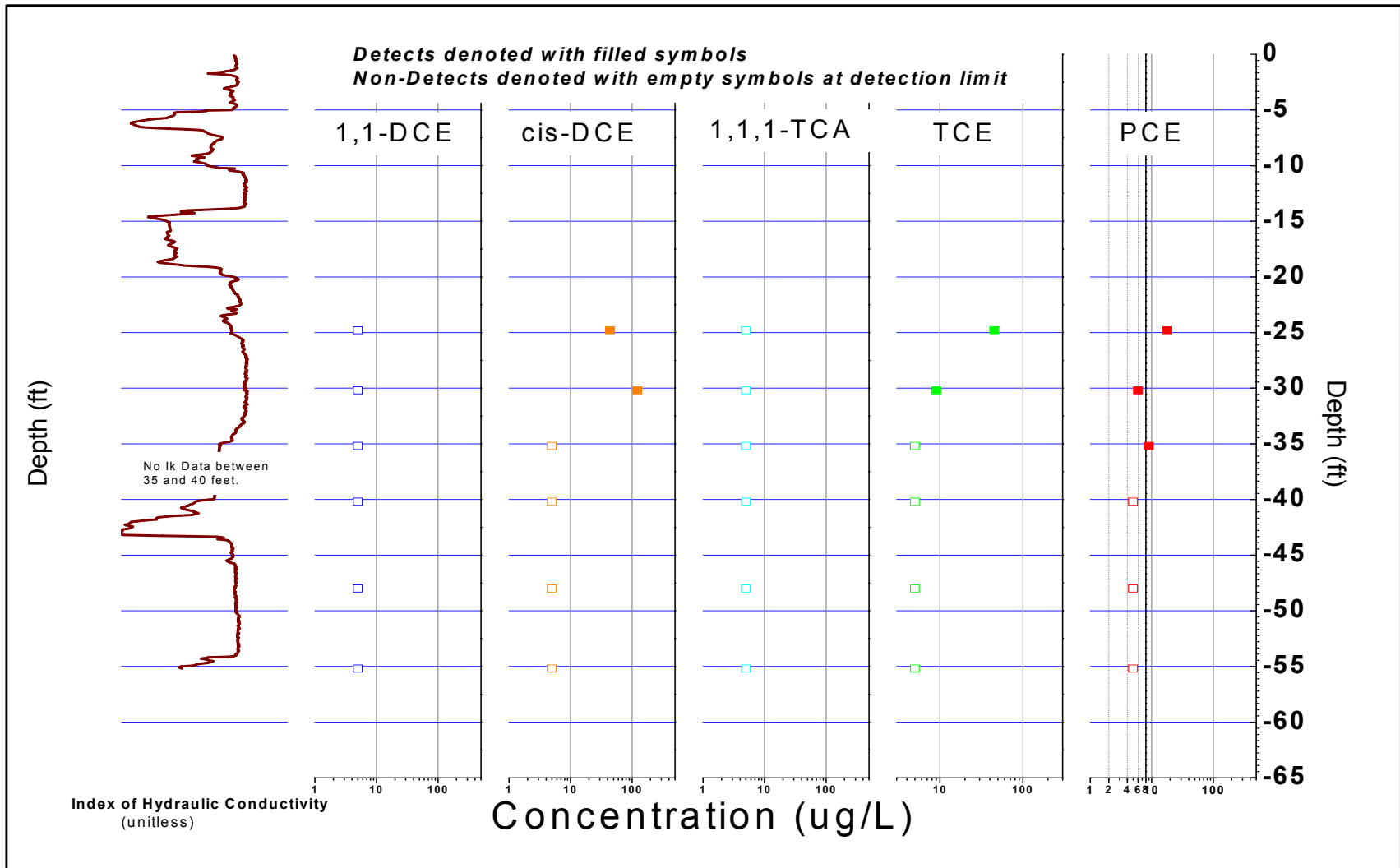
FIGURE B-225, I_k RECORD AND SELECTED VOC ANALYTICAL RESULTS ERM, Wayland, Massachusetts
