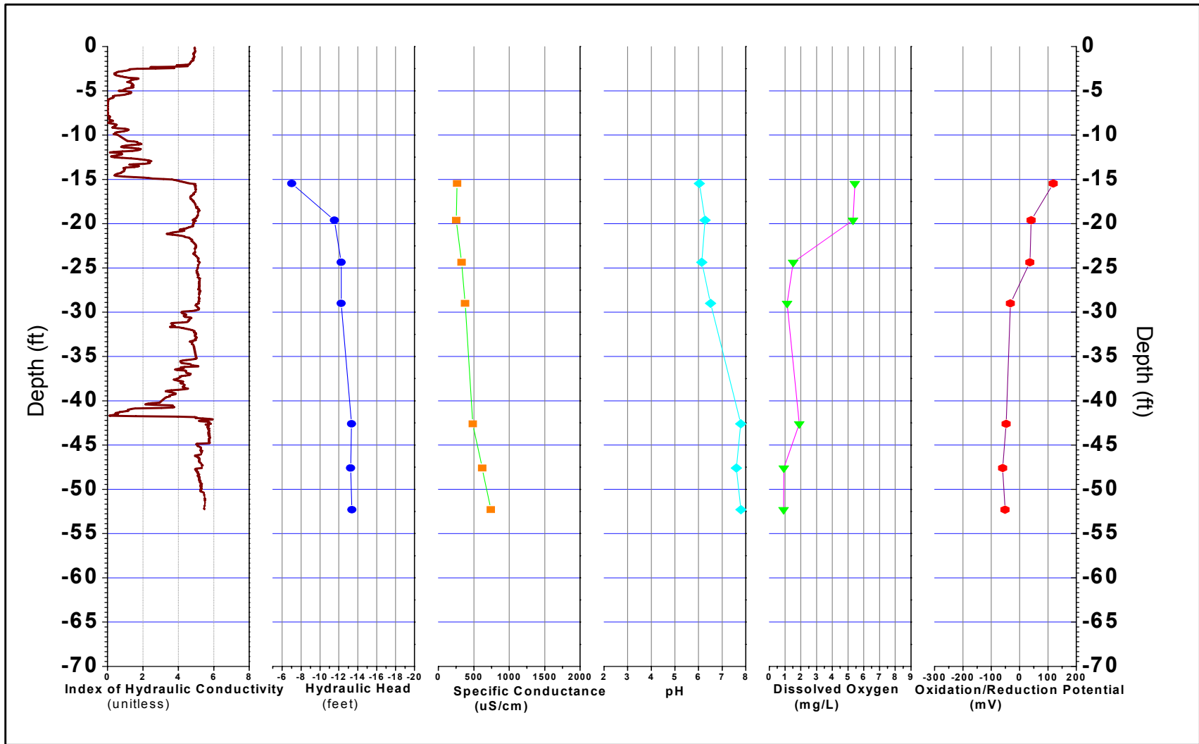
FIGURE B-234, I_k RECORD AND PHYSICO-CHEMICAL PARAMETERS ERM, Wayland, Massachusetts
