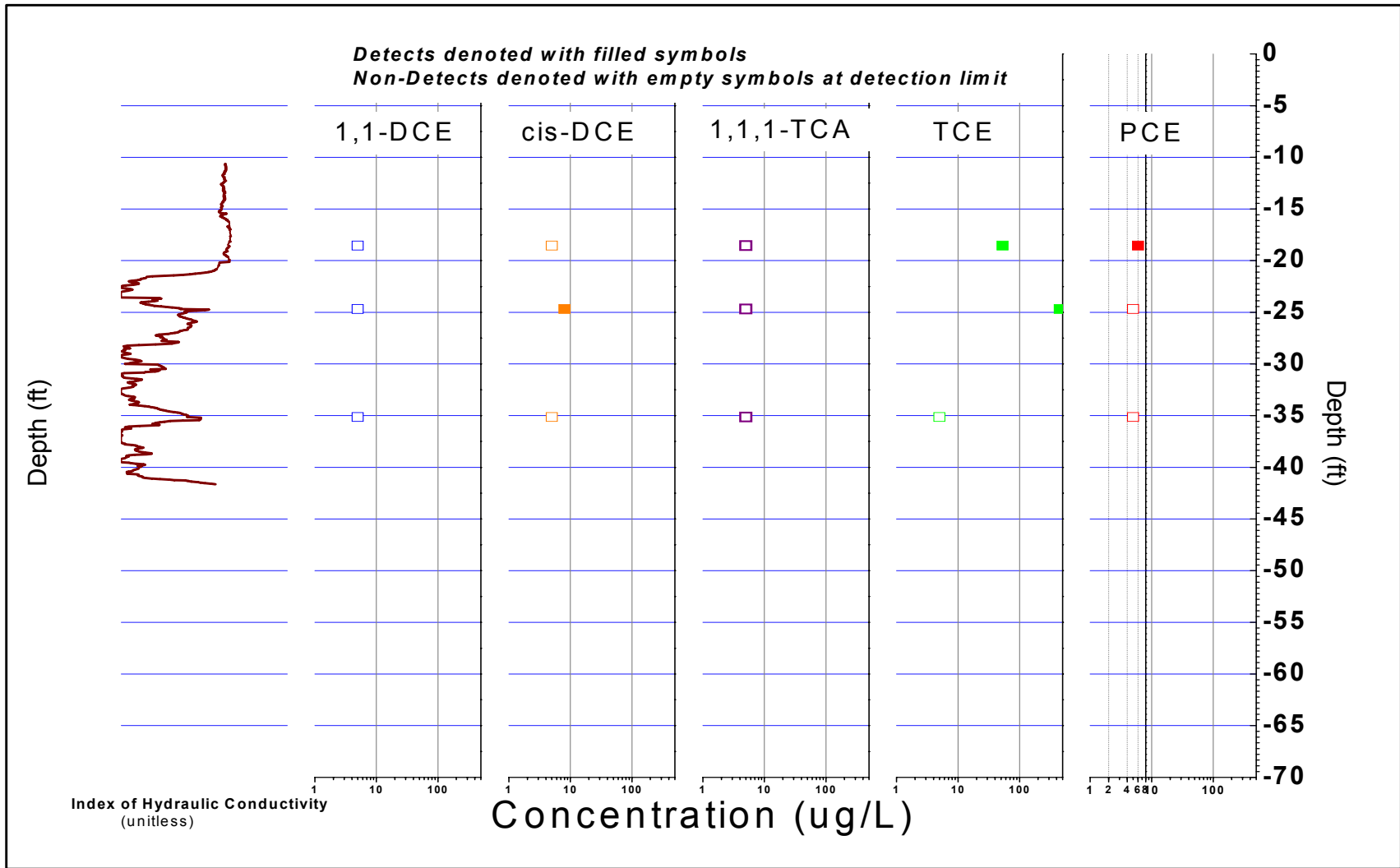
FIGURE B-201, I k RECORD AND SELECTED VOC ANALYTICAL RESULTS ERM, Wayland, Massachusetts
