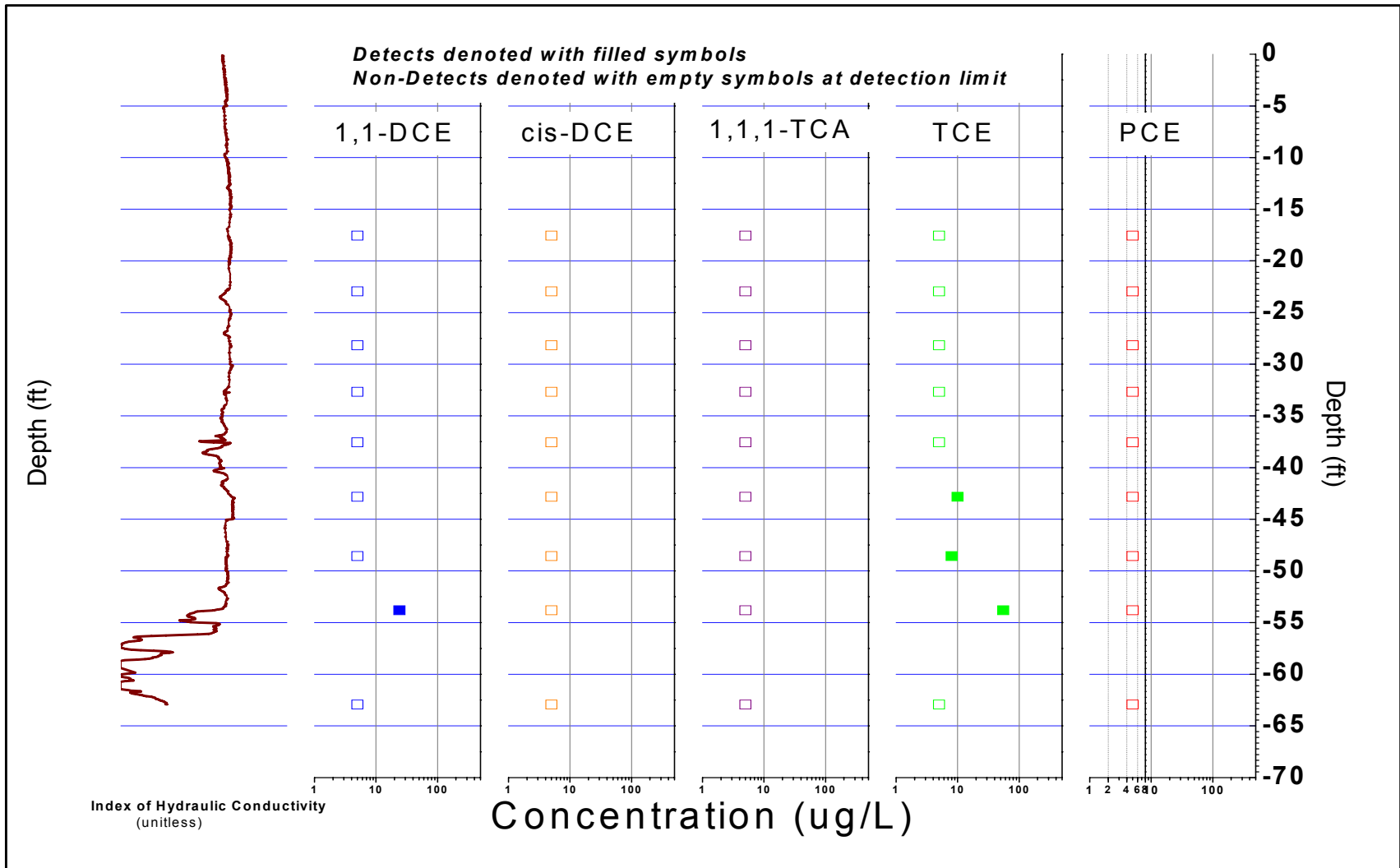
FIGURE B-206, I_k RECORD AND SELECTED VOC ANALYTICAL RESULTS ERM, Wayland, Massachusetts
