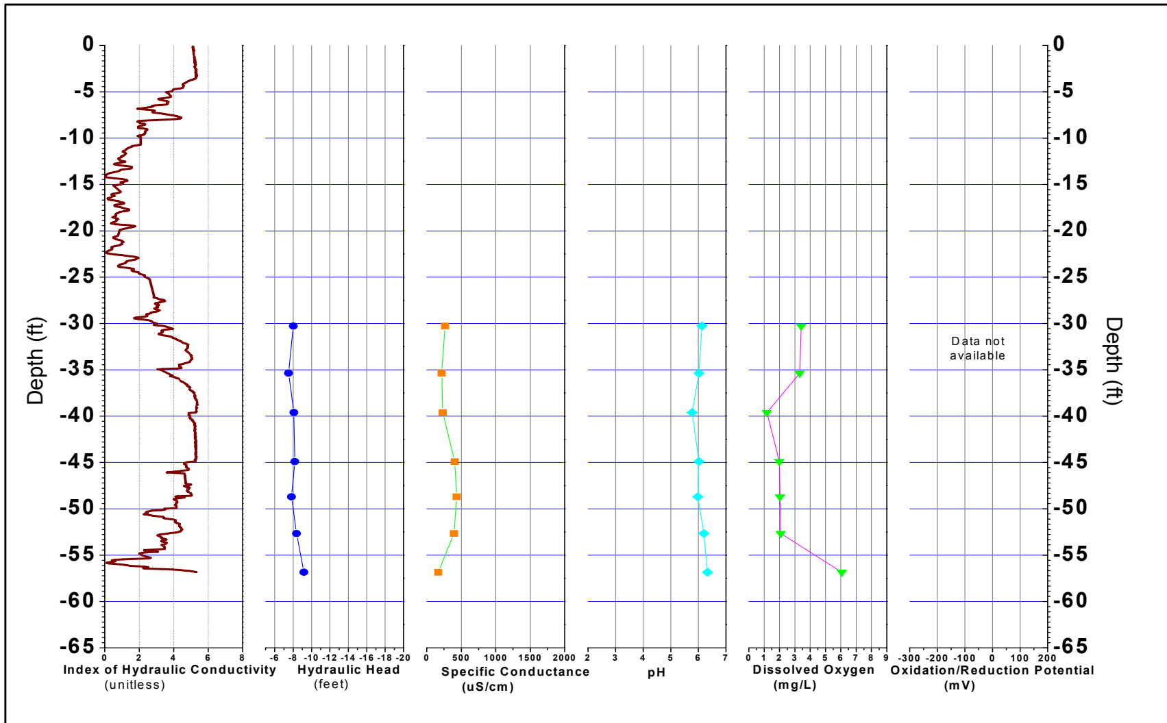
FIGURE B-226, I k RECORD AND PHYSICO-CHEMICAL PARAMETERS ERM, Wayland, Massachusetts
