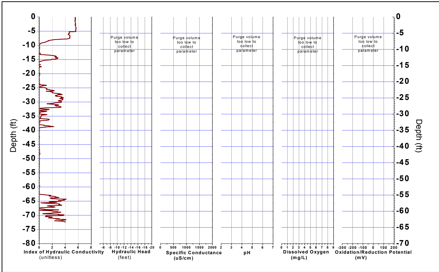
FIGURE B-239, I_k RECORD AND PHYSICO-CHEMICAL PARAMETERS ERM, Wayland, Massachusetts
