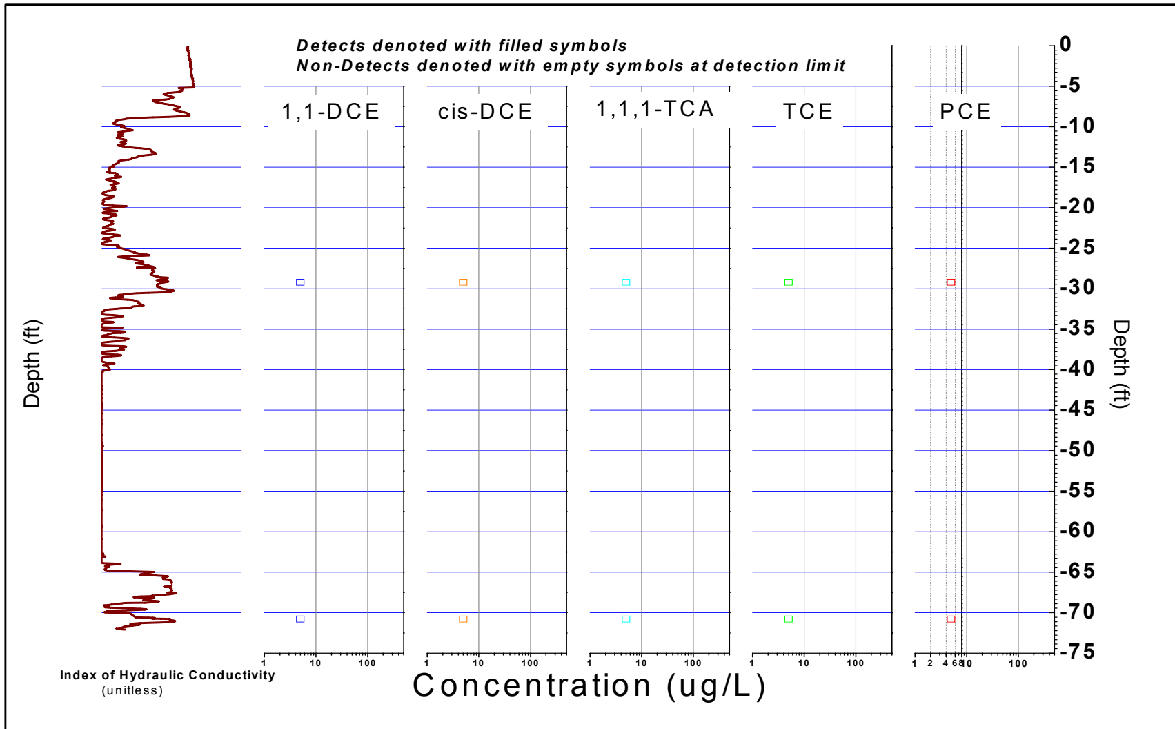
FIGURE B-237, I k RECORD AND SELECTED VOC ANALYTICAL RESULTS ERM, Wayland, Massachusetts
