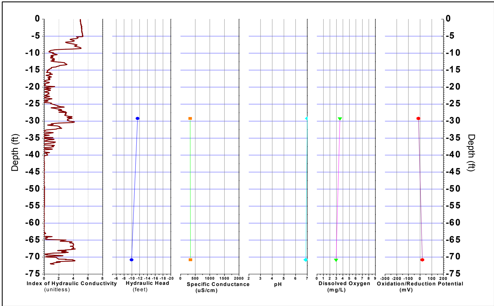
FIGURE B-237, I_k RECORD AND PHYSICO-CHEMICAL PARAMETERS ERM, Wayland, Massachusetts
