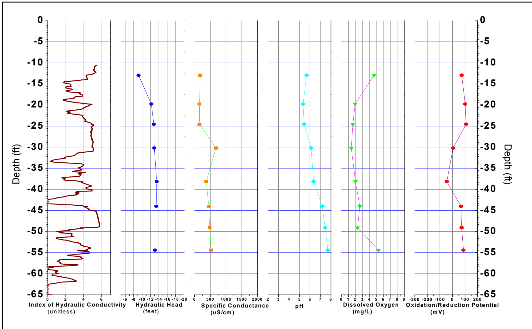
FIGURE B-221, I_k RECORD AND PHYSICO-CHEMICAL PARAMETERS ERM, Wayland, Massachusetts
