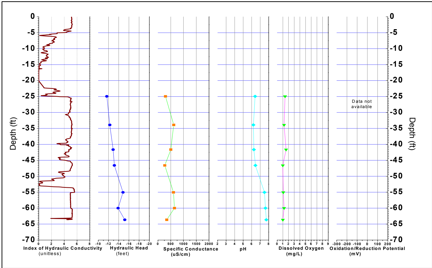
FIGURE B-236, I k RECORD AND PHYSICO-CHEMICAL PARAMETERS ERM, Wayland, Massachusetts
