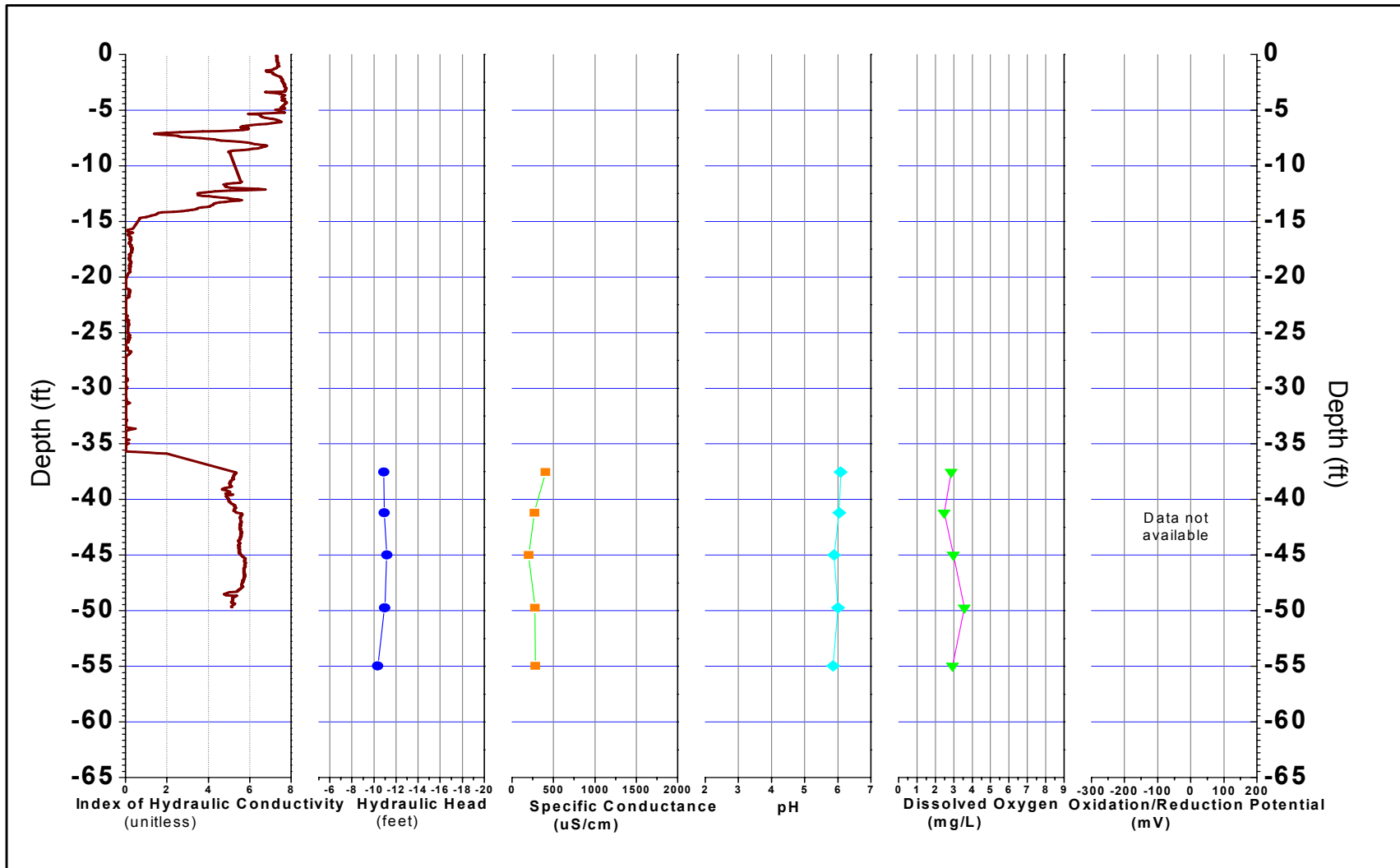
FIGURE B-227, I_k RECORD AND PHYSICO-CHEMICAL PARAMETERS ERM, Wayland, Massachusetts
