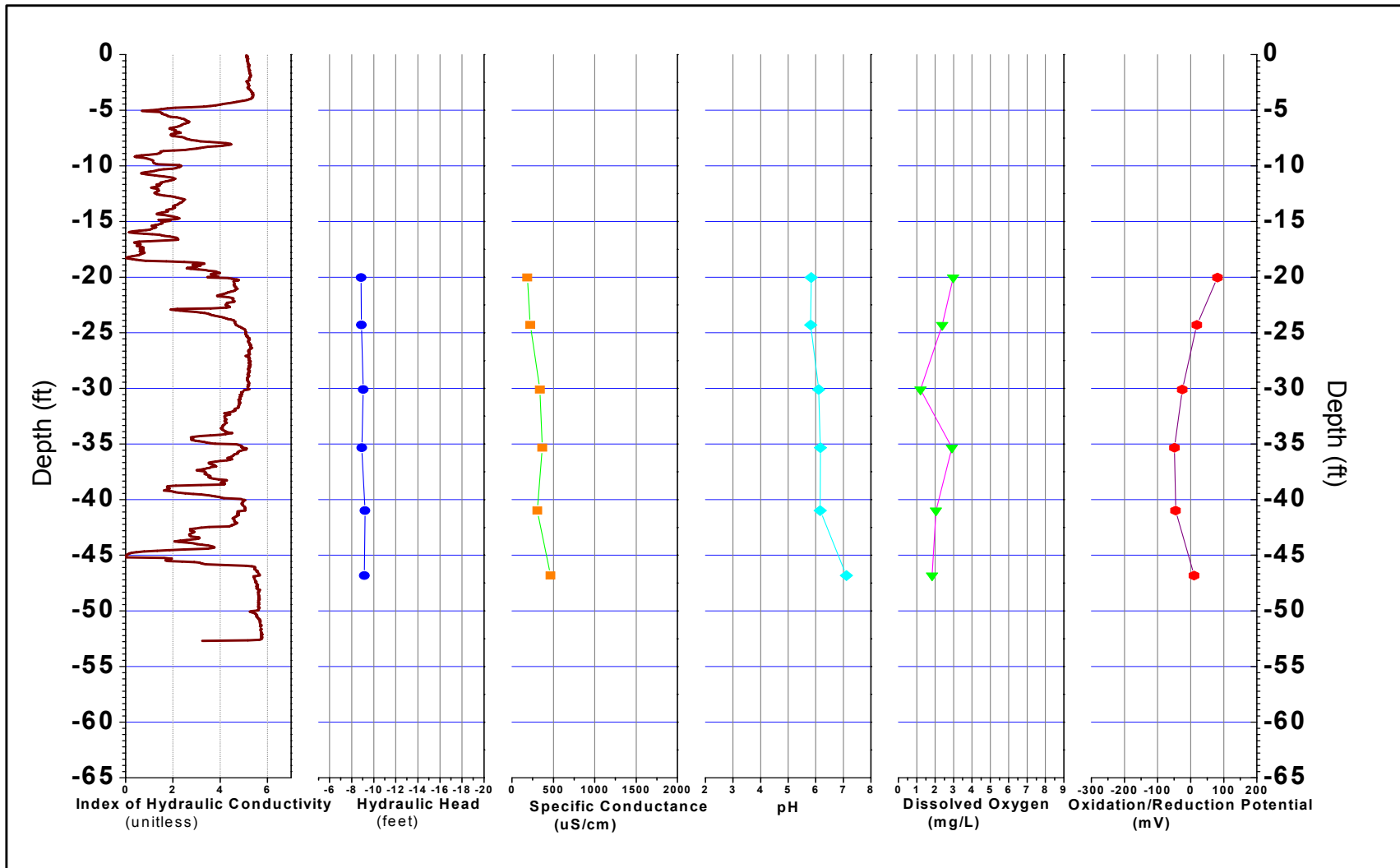
FIGURE B-223, I_k RECORD AND PHYSICO-CHEMICAL PARAMETERS ERM, Wayland, Massachusetts
