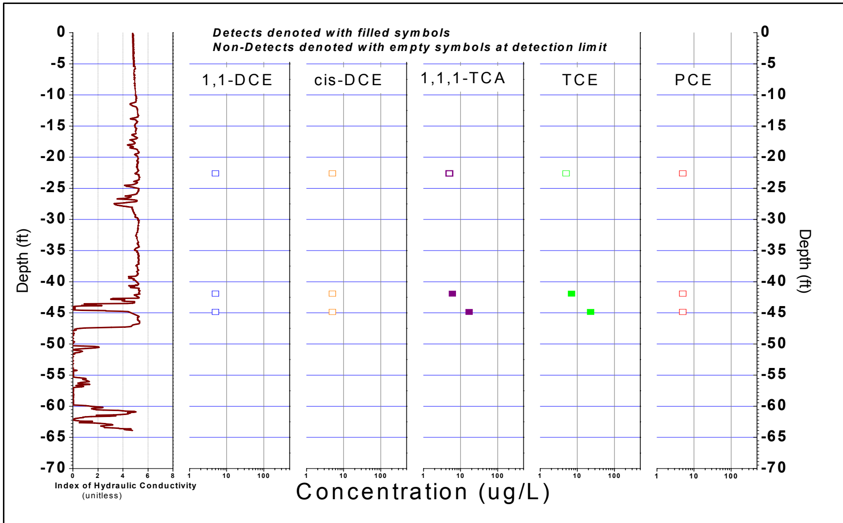
FIGURE B-205, I_k RECORD AND SELECTED VOC ANALYTICAL RESULTS ERM, Wayland, Massachusetts
