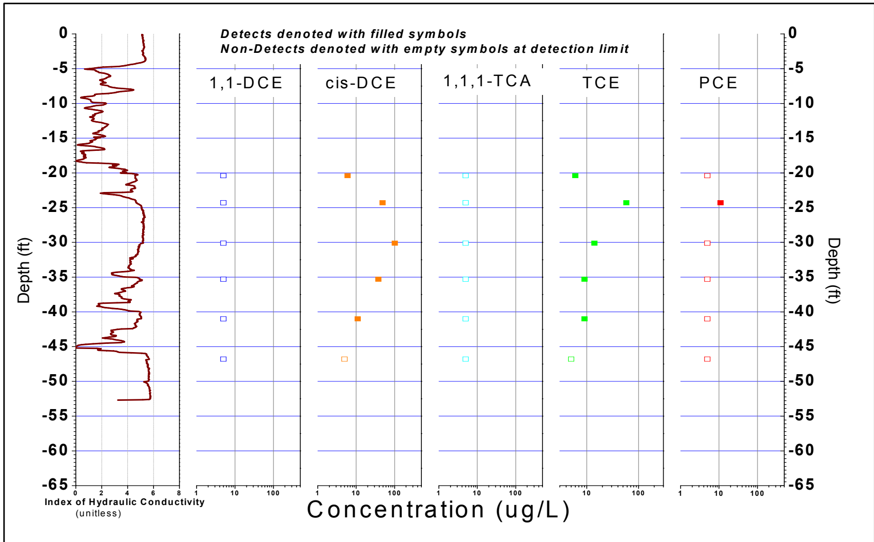
FIGURE B-223, I_k RECORD AND SELECTED VOC ANALYTICAL RESULTS ERM, Wayland, Massachusetts
