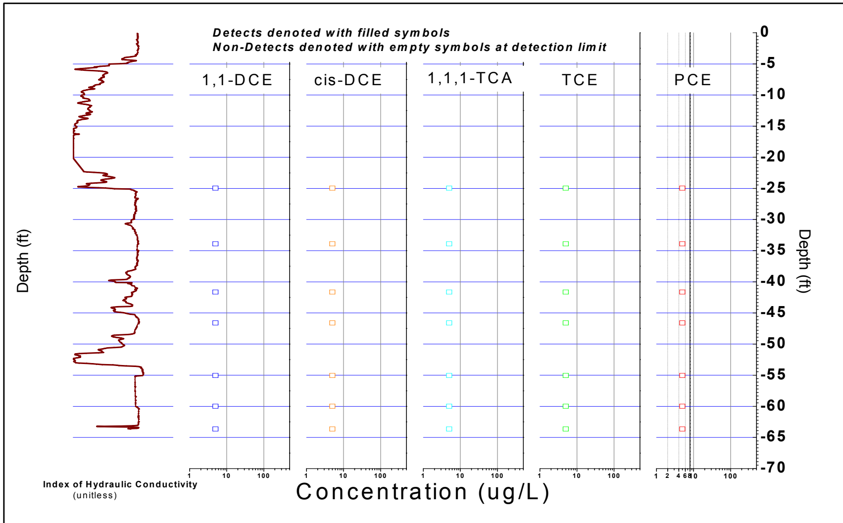
FIGURE B-236, I k RECORD AND SELECTED VOC ANALYTICAL RESULTS ERM, Wayland, Massachusetts
