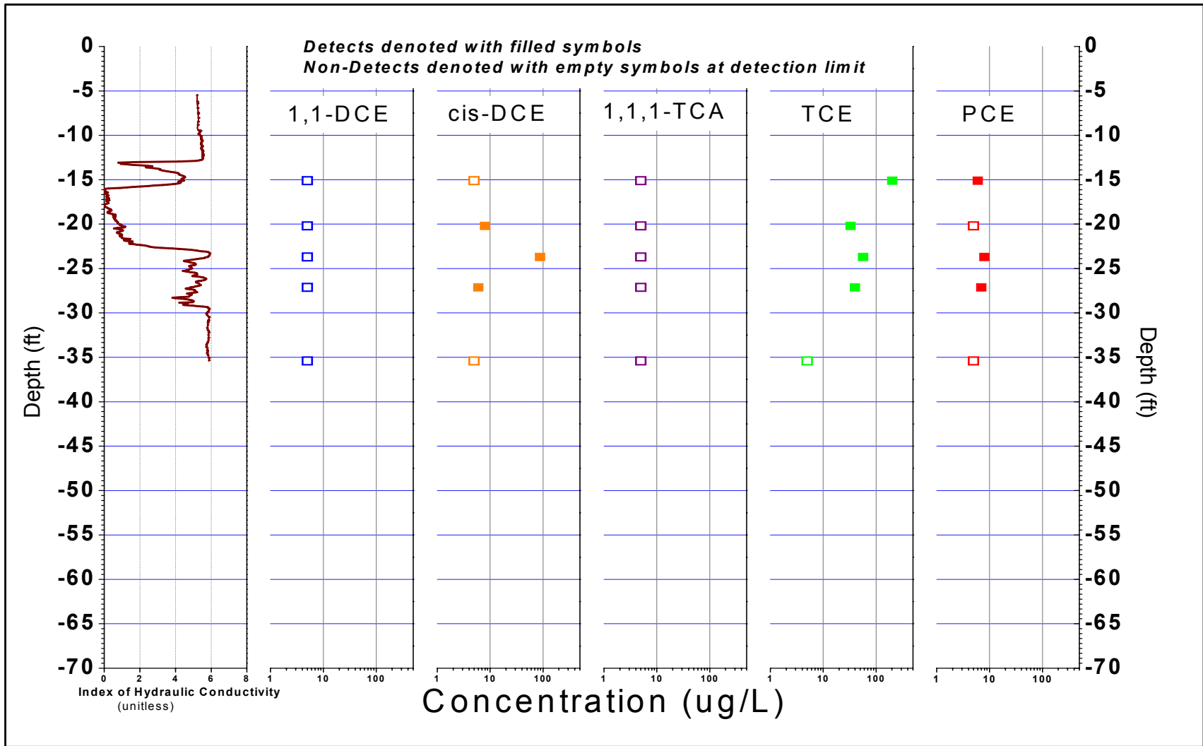
FIGURE B-210, I k RECORD AND SELECTED VOC ANALYTICAL RESULTS ERM, Wayland, Massachusetts
