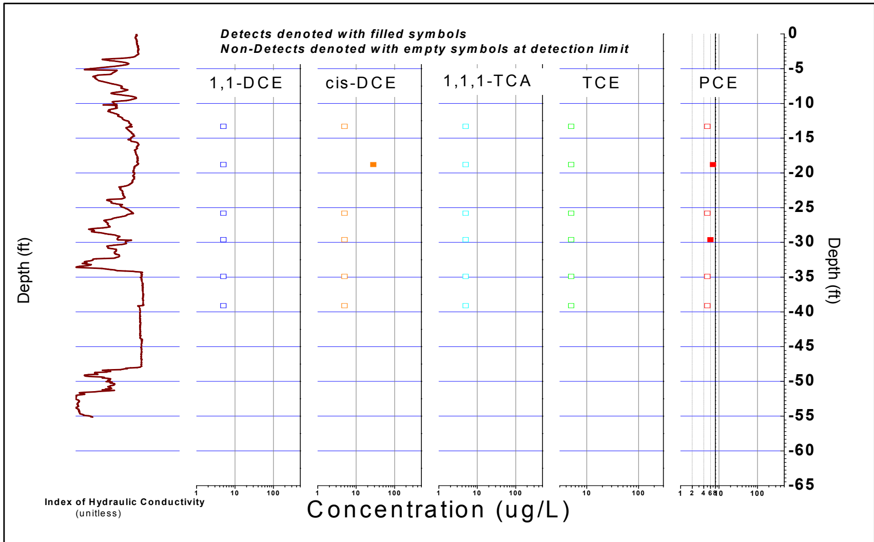
FIGURE B-224, I_k RECORD AND SELECTED VOC ANALYTICAL RESULTS ERM, Wayland, Massachusetts
