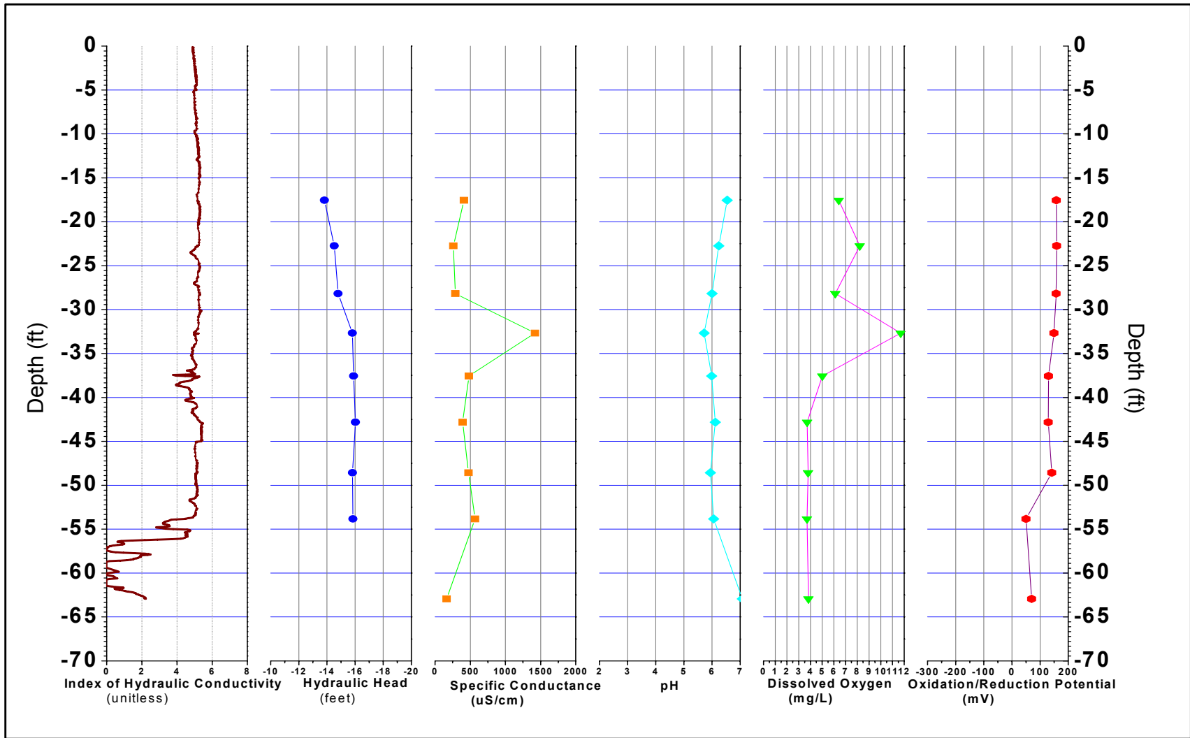
FIGURE B-206, I k RECORD AND PHYSICO-CHEMICAL PARAMETERS ERM, Wayland, Massachusetts
