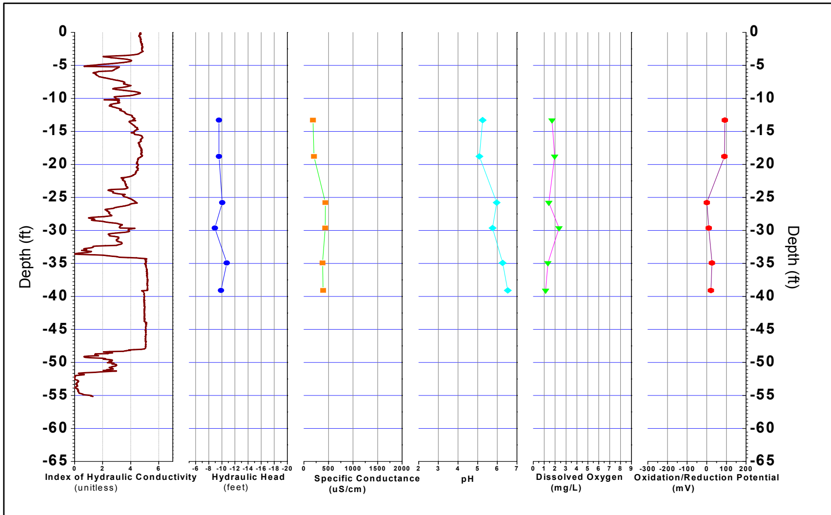
FIGURE B-224, I_K RECORD AND PHYSICO-CHEMICAL PARAMETERS ERM, Wayland, Massachusetts
