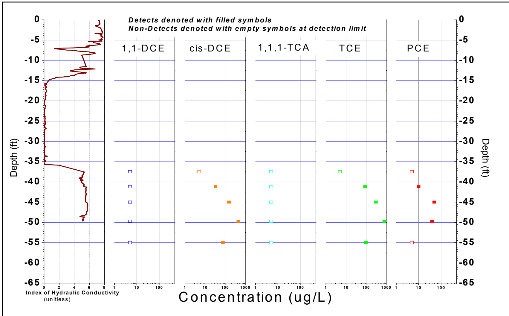
FIGURE B-227, I_k RECORD AND SELECTED VOC ANALYTICAL RESULTS ERM, Wayland, Massachusetts
