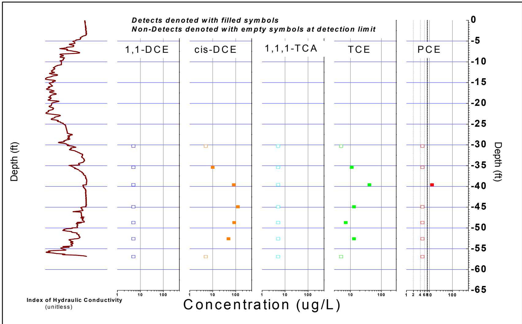
FIGURE B-226, I_k RECORD AND SELECTED VOC ANALYTICAL RESULTS ERM, Wayland, Massachusetts
