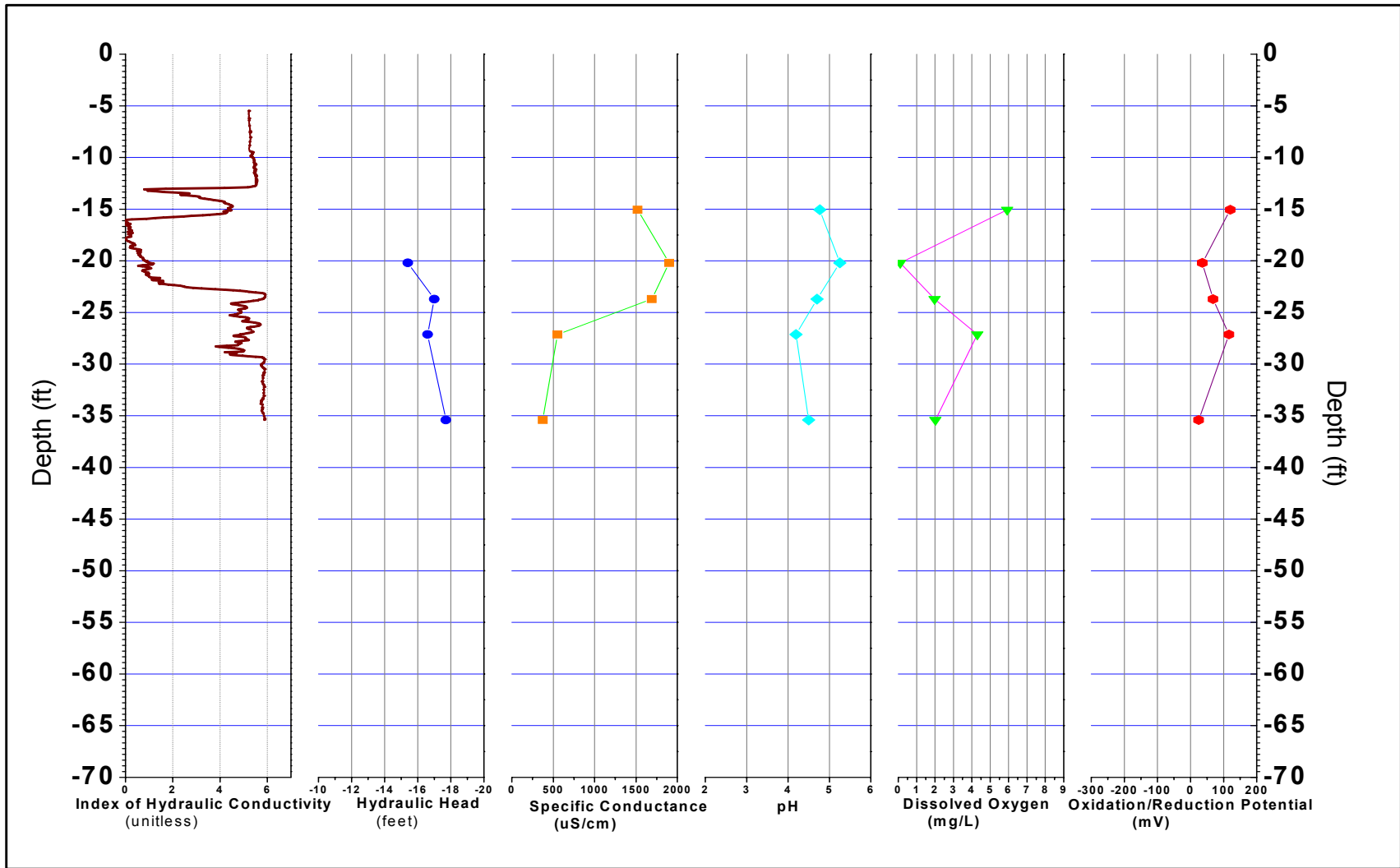
FIGURE B-210, I k RECORD AND PHYSICO-CHEMICAL PARAMETERS ERM, Wayland, Massachusetts
