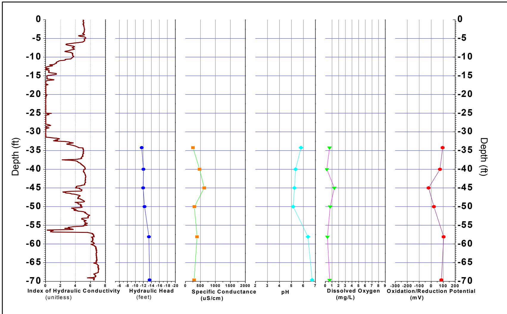
FIGURE B-231, I_k RECORD AND PHYSICO-CHEMICAL PARAMETERS ERM, Wayland, Massachusetts
