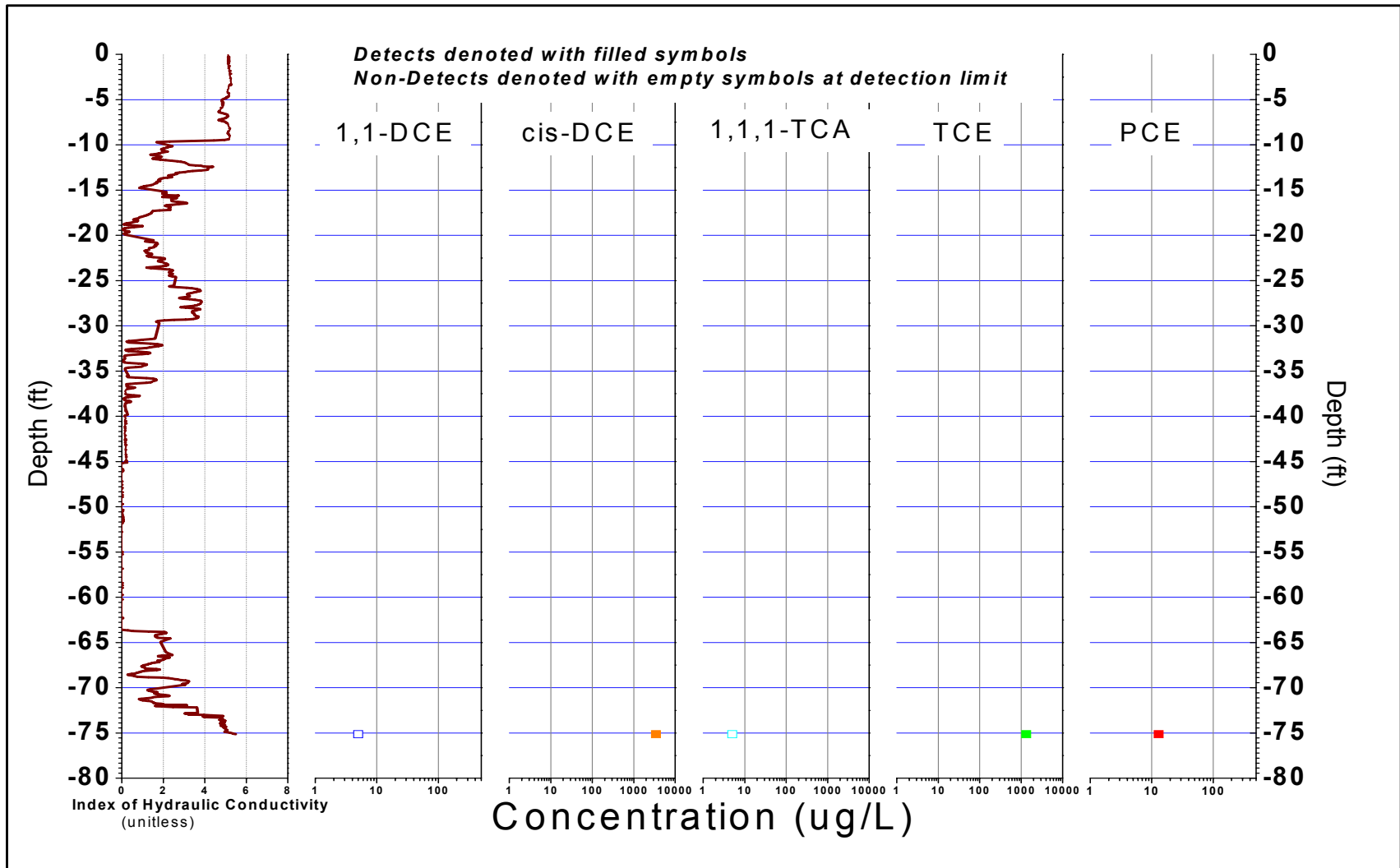
FIGURE B-232, I K RECORD AND SELECTED VOC ANALYTICAL RESULTS ERM, Wayland, Massachusetts
