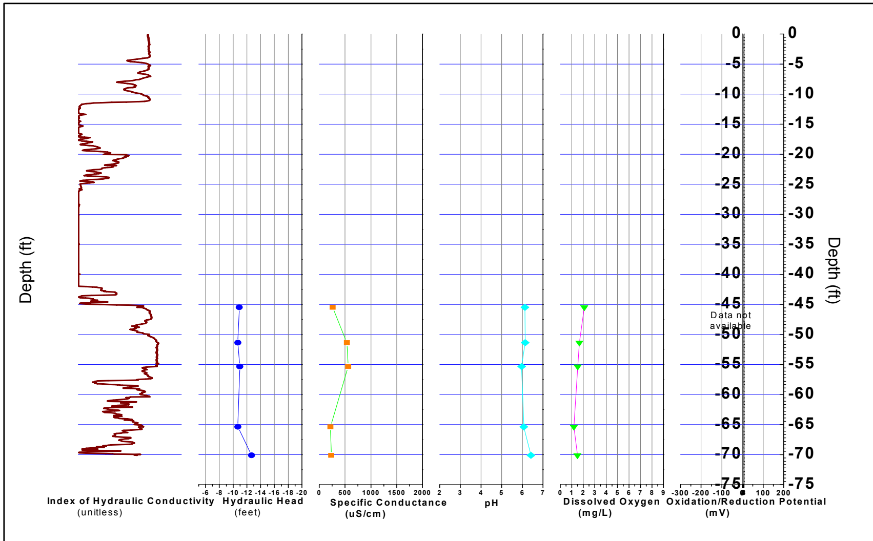
FIGURE B-230, I k RECORD AND PHYSICO-CHEMICAL PARAMETERS ERM, Wayland, Massachusetts
