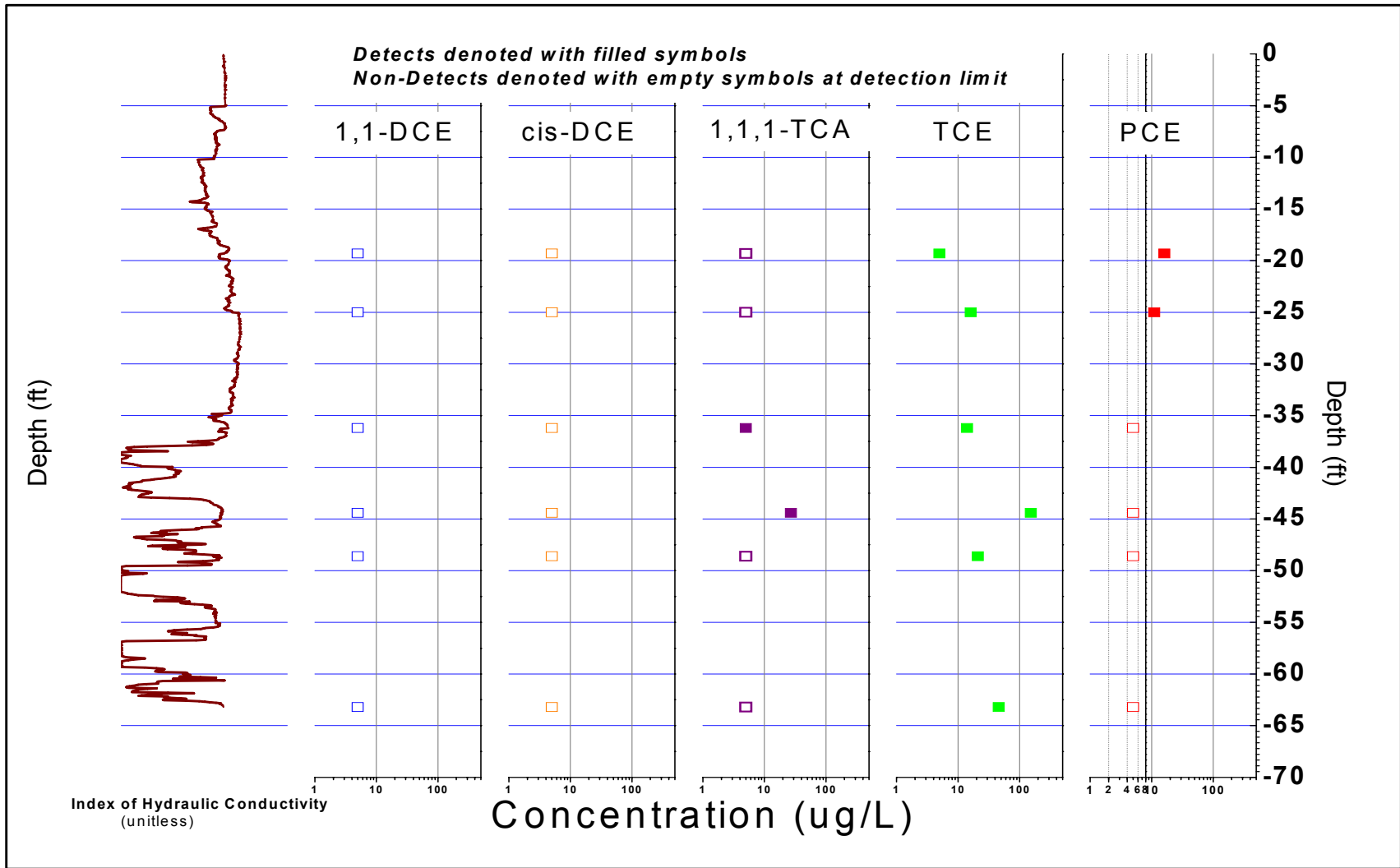
FIGURE B-204, I k RECORD AND SELECTED VOC ANALYTICAL RESULTS ERM, Wayland, Massachusetts
