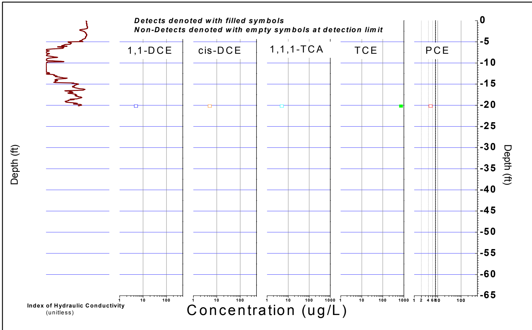
FIGURE B-242, I_K RECORD AND SELECTED VOC ANALYTICAL RESULTS ERM, Wayland, Massachusetts
