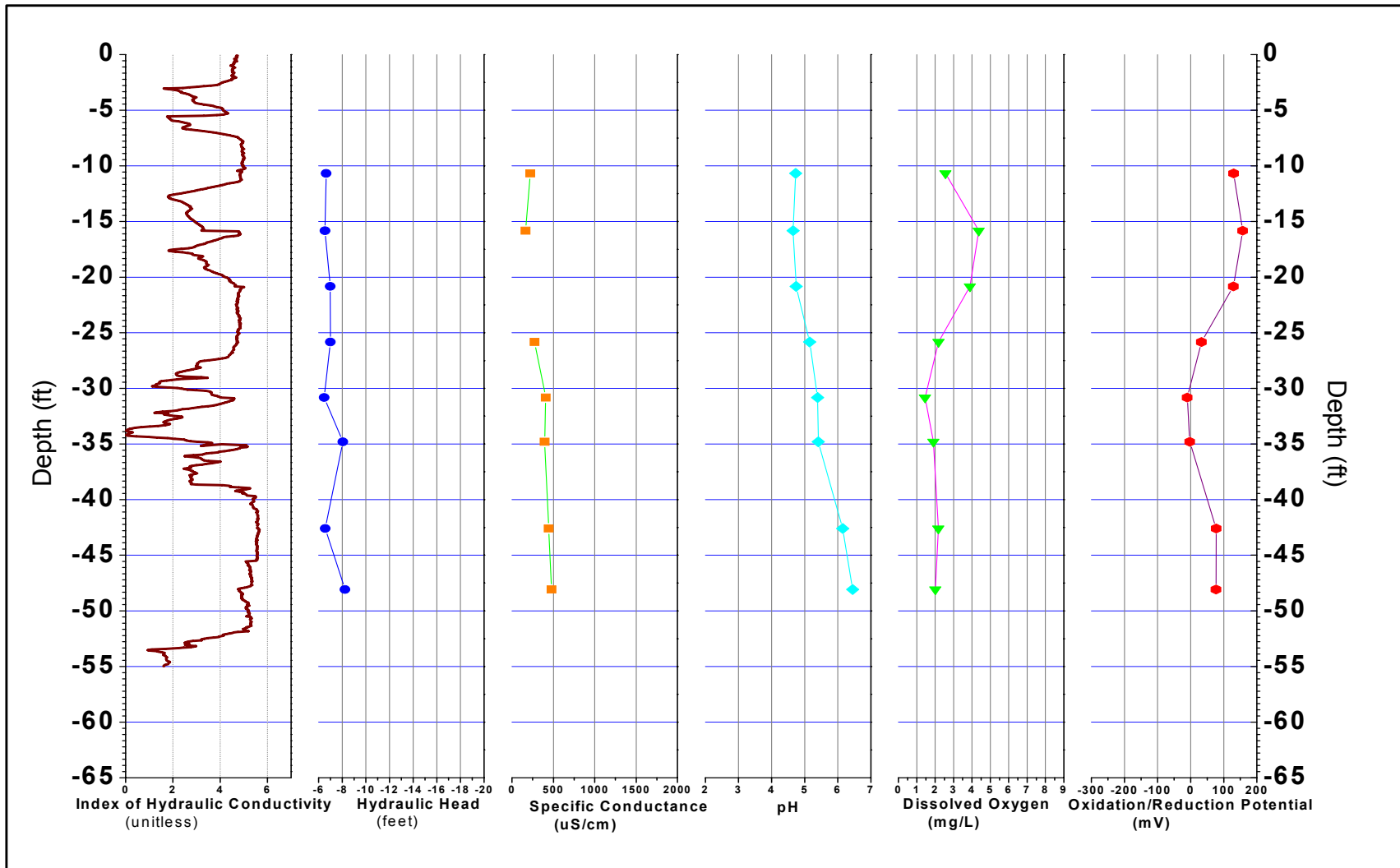
FIGURE B-222, I_k RECORD AND PHYSICO-CHEMICAL PARAMETERS ERM, Wayland, Massachusetts
