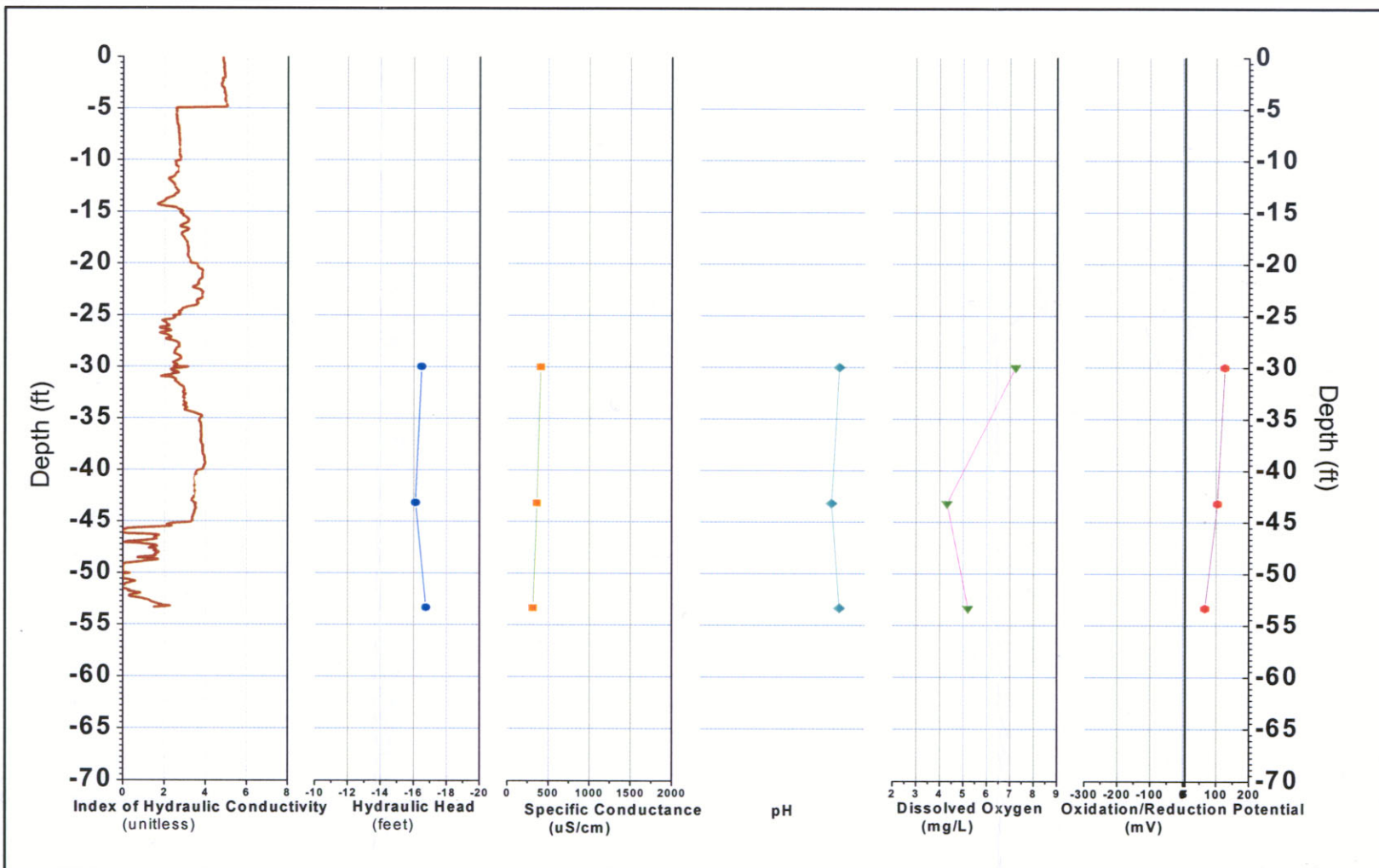
FIGURE B-203, I k RECORD AND PHYSICO-CHEMICAL PARAMETERS ERM, Wayland, Massachusetts
