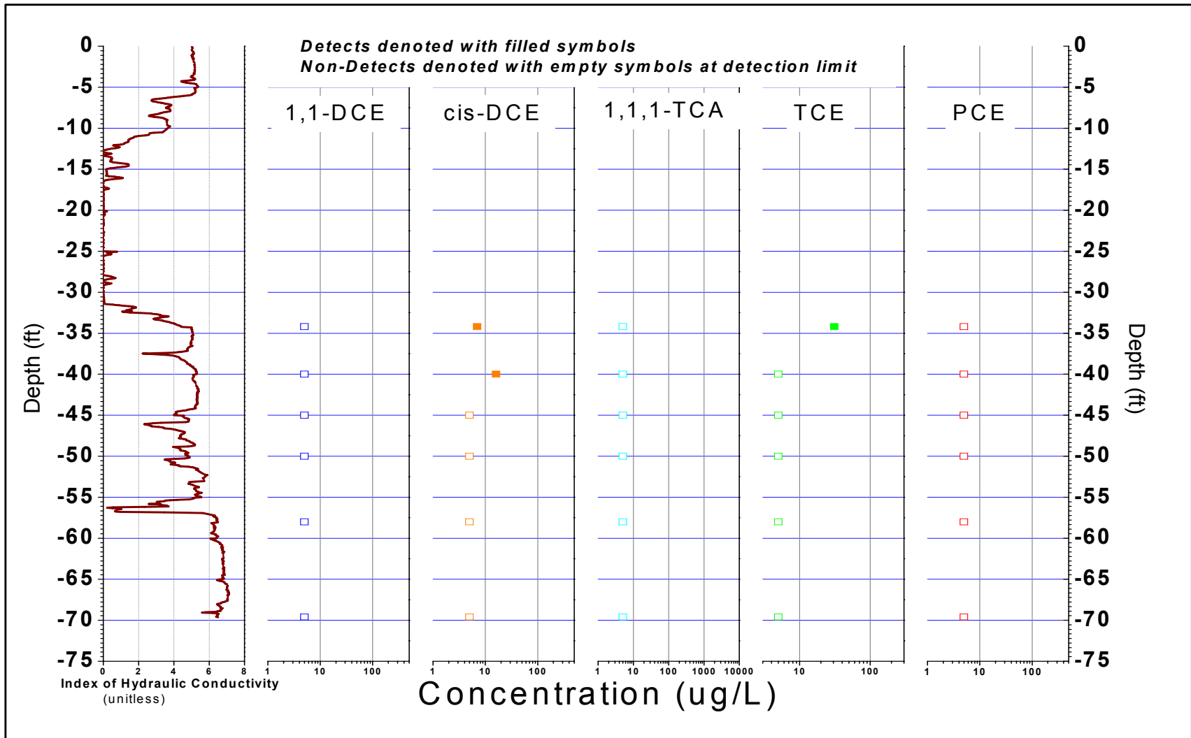
FIGURE B-231, I_k RECORD AND SELECTED VOC ANALYTICAL RESULTS ERM, Wayland, Massachusetts
