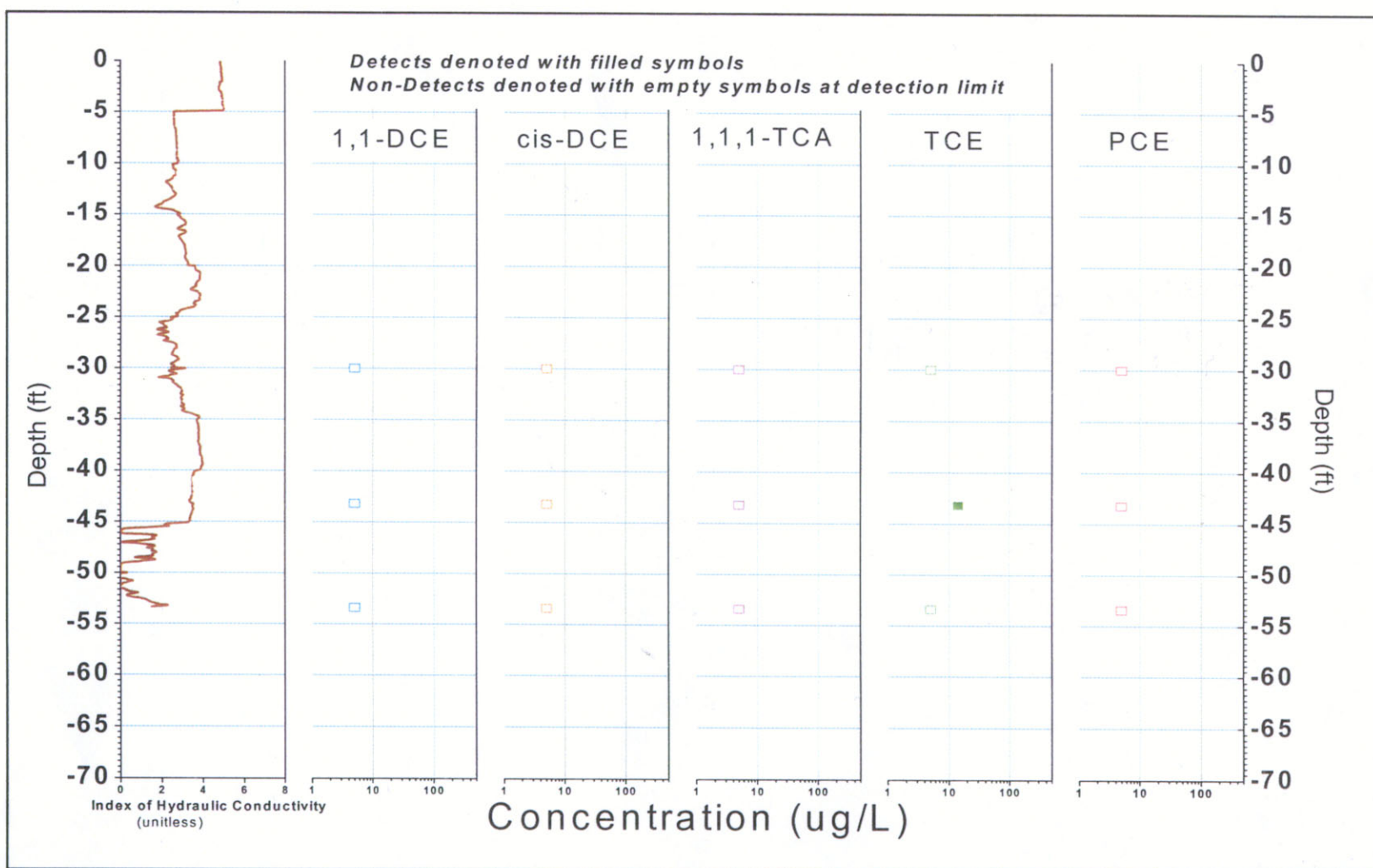
FIGURE B-203, I k RECORD AND SELECTED VOC ANALYTICAL RESULTS ERM, Wayland, Massachusetts
