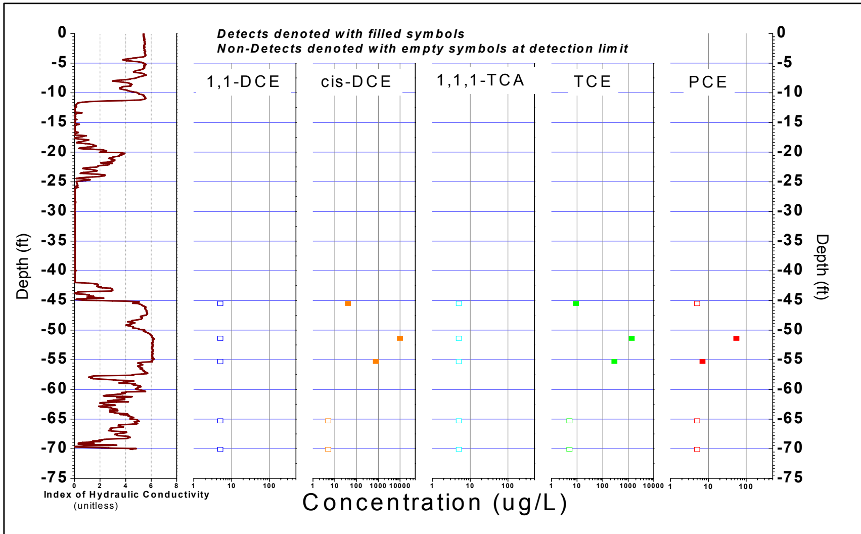
FIGURE B-230, I_k RECORD AND SELECTED VOC ANALYTICAL RESULTS ERM, Wayland, Massachusetts
