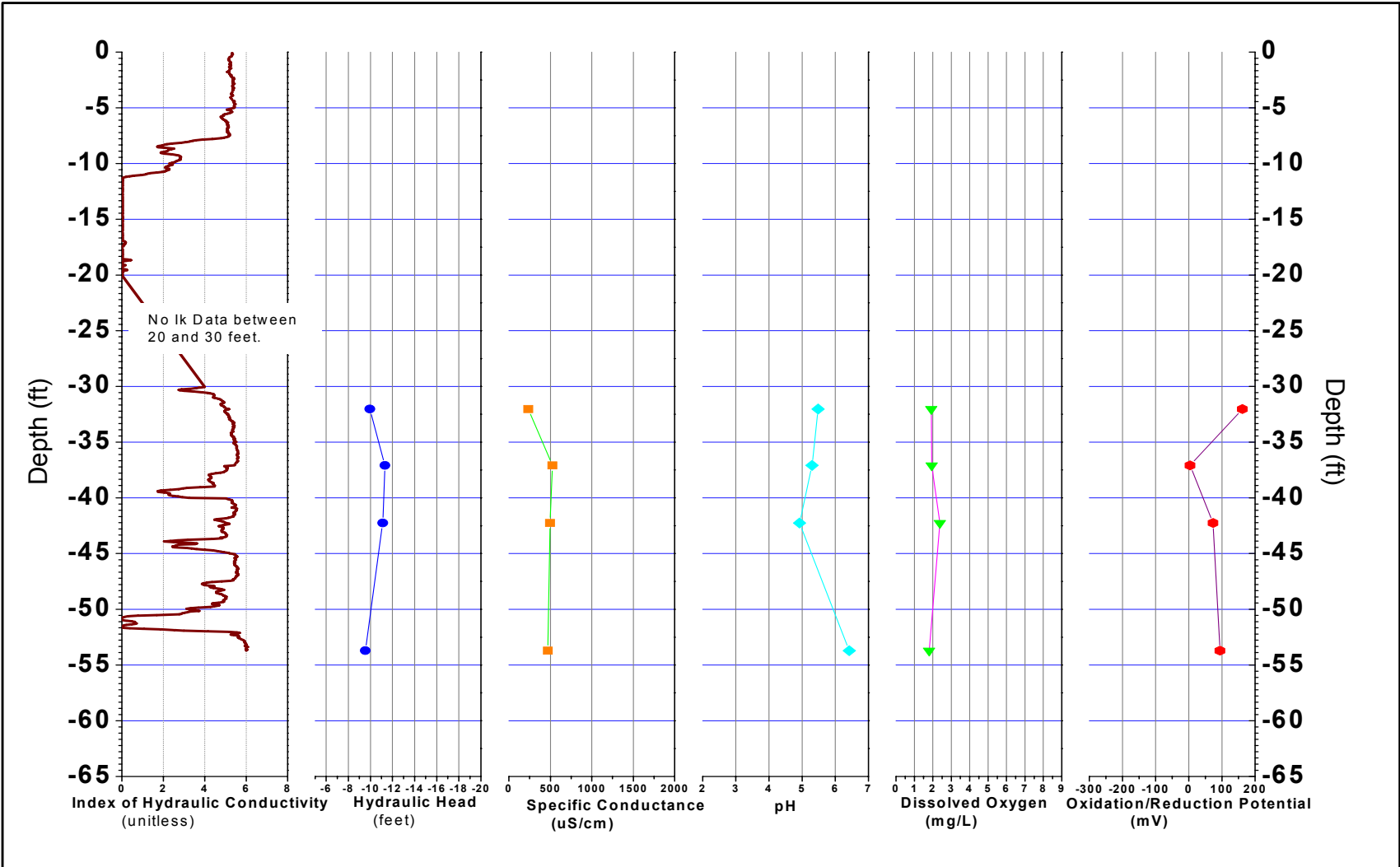
FIGURE B-229, I_k RECORD AND PHYSICO-CHEMICAL PARAMETERS ERM, Wayland, Massachusetts
