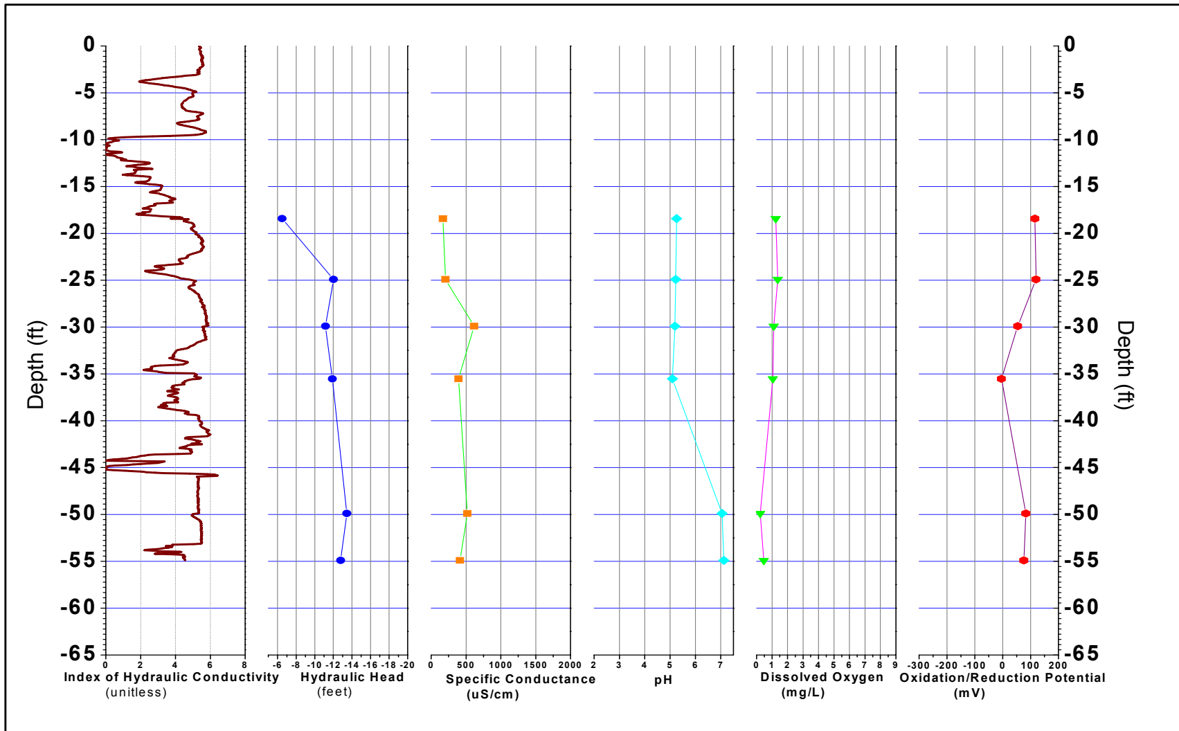
FIGURE B-228, I_k RECORD AND PHYSICO-CHEMICAL PARAMETERS ERM, Wayland, Massachusetts
