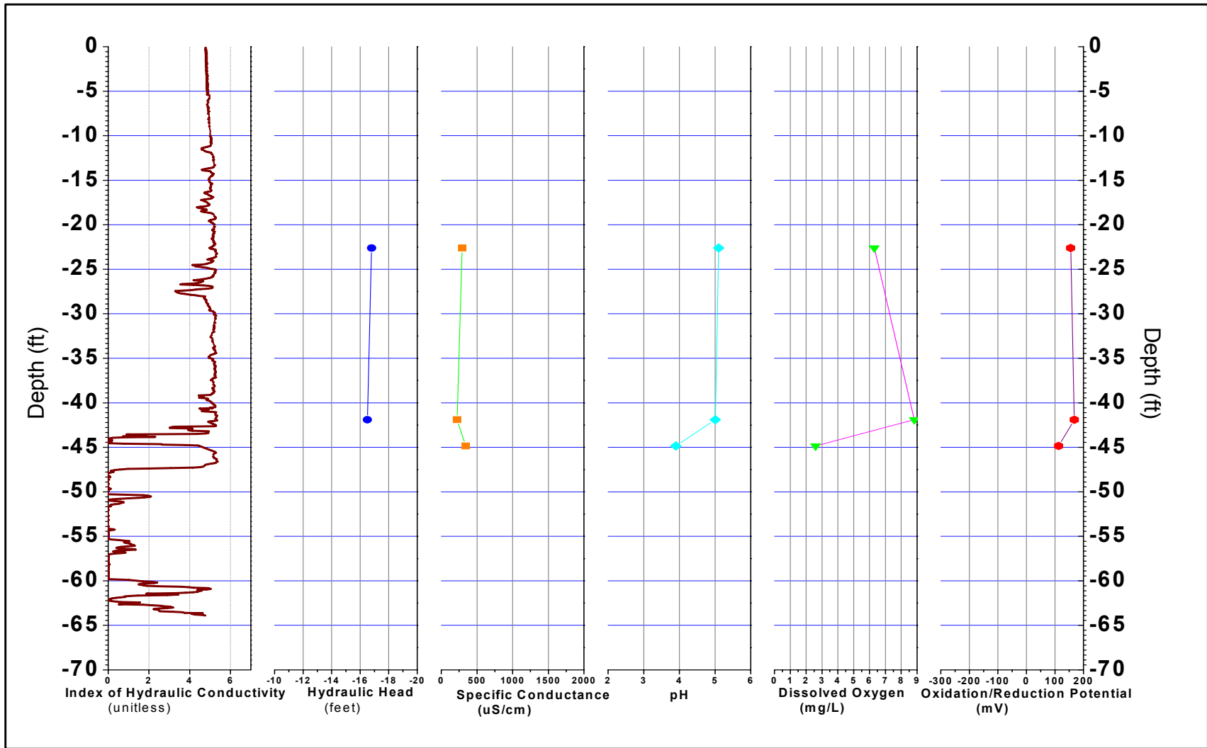
FIGURE B-205, I k RECORD AND PHYSICO-CHEMICAL PARAMETERS ERM, Wayland, Massachusetts
