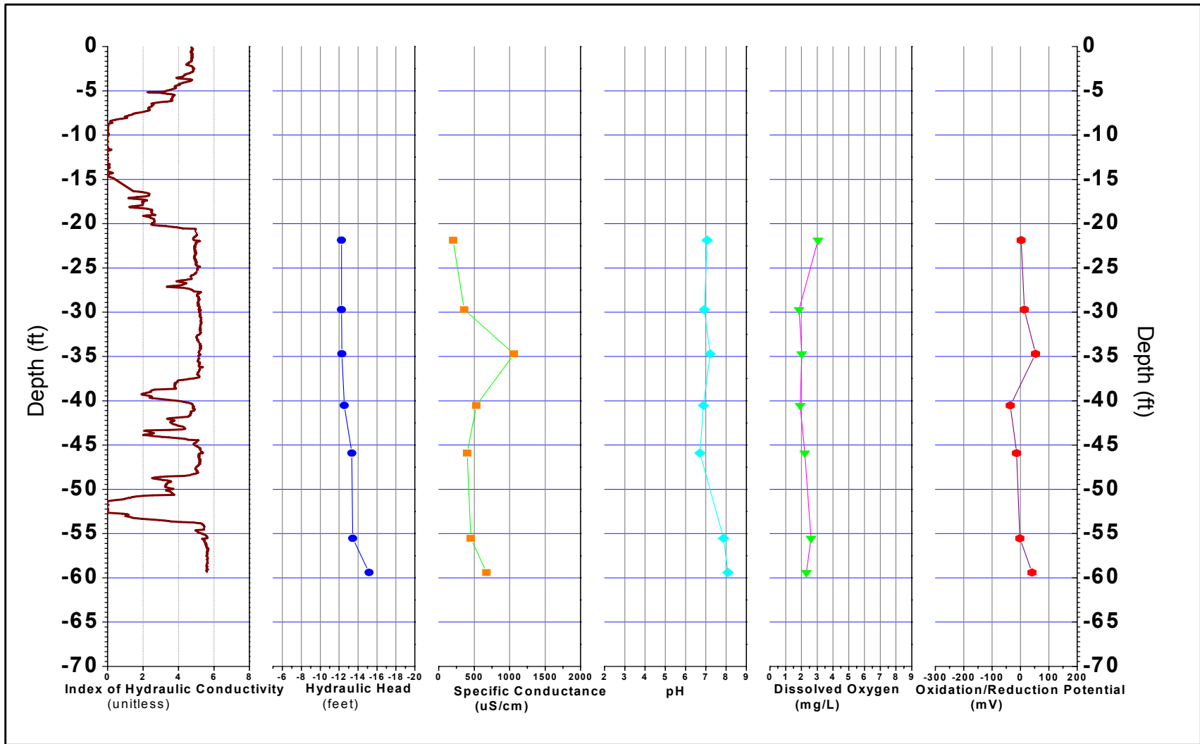
FIGURE B-235, I_k RECORD AND PHYSICO-CHEMICAL PARAMETERS ERM, Wayland, Massachusetts
