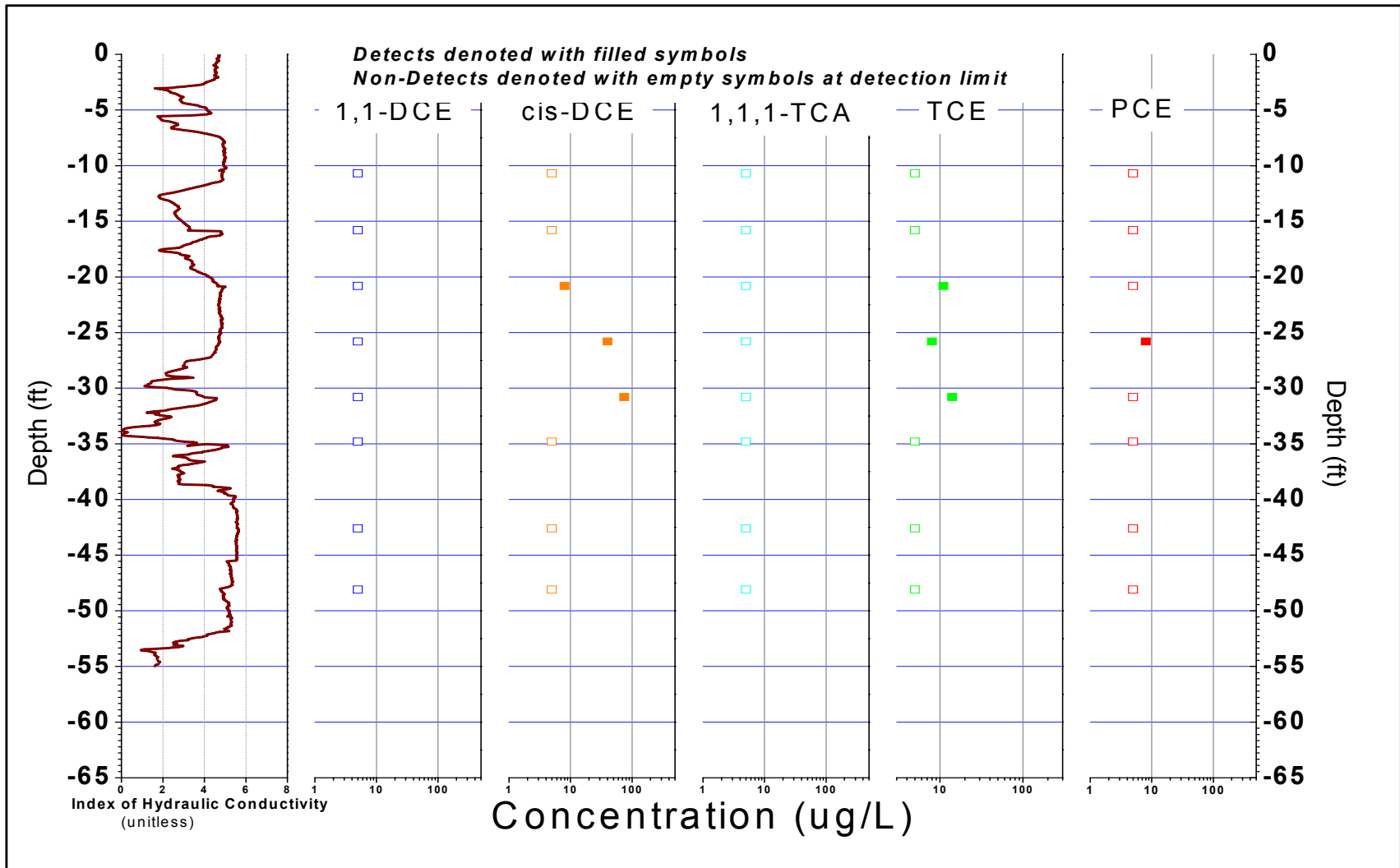
FIGURE B-222, I_k RECORD AND SELECTED VOC ANALYTICAL RESULTS ERM, Wayland, Massachusetts
