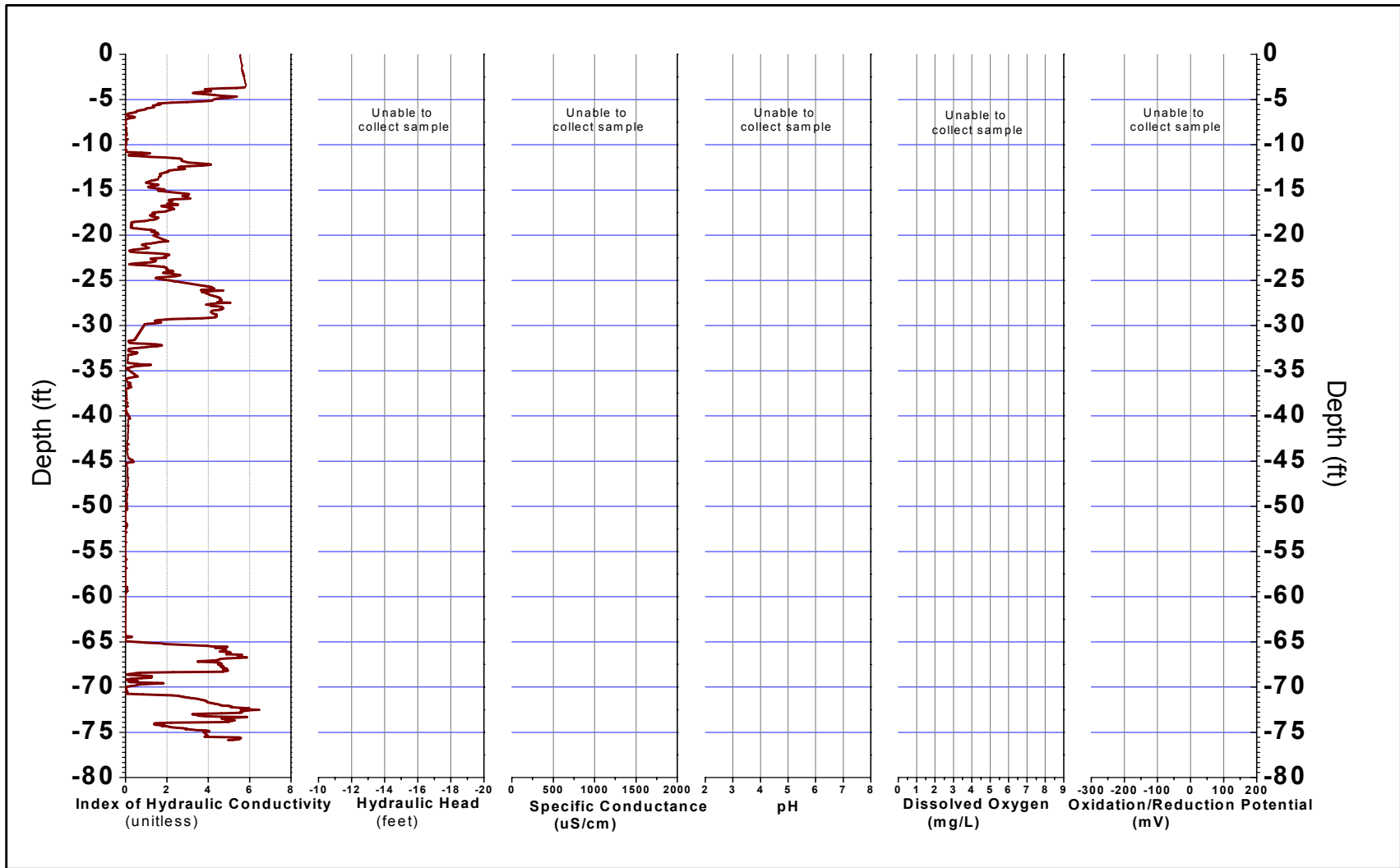
FIGURE B-238, I_k RECORD AND PHYSICO-CHEMICAL PARAMETERS ERM, Wayland, Massachusetts
