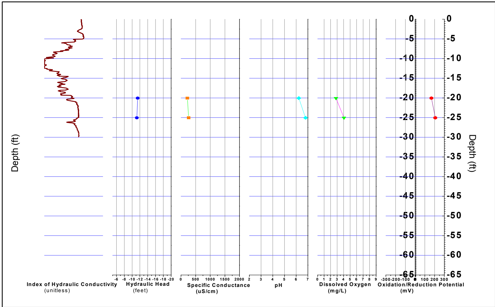
FIGURE B-241, I_k RECORD AND PHYSICO-CHEMICAL PARAMETERS ERM, Wayland, Massachusetts
