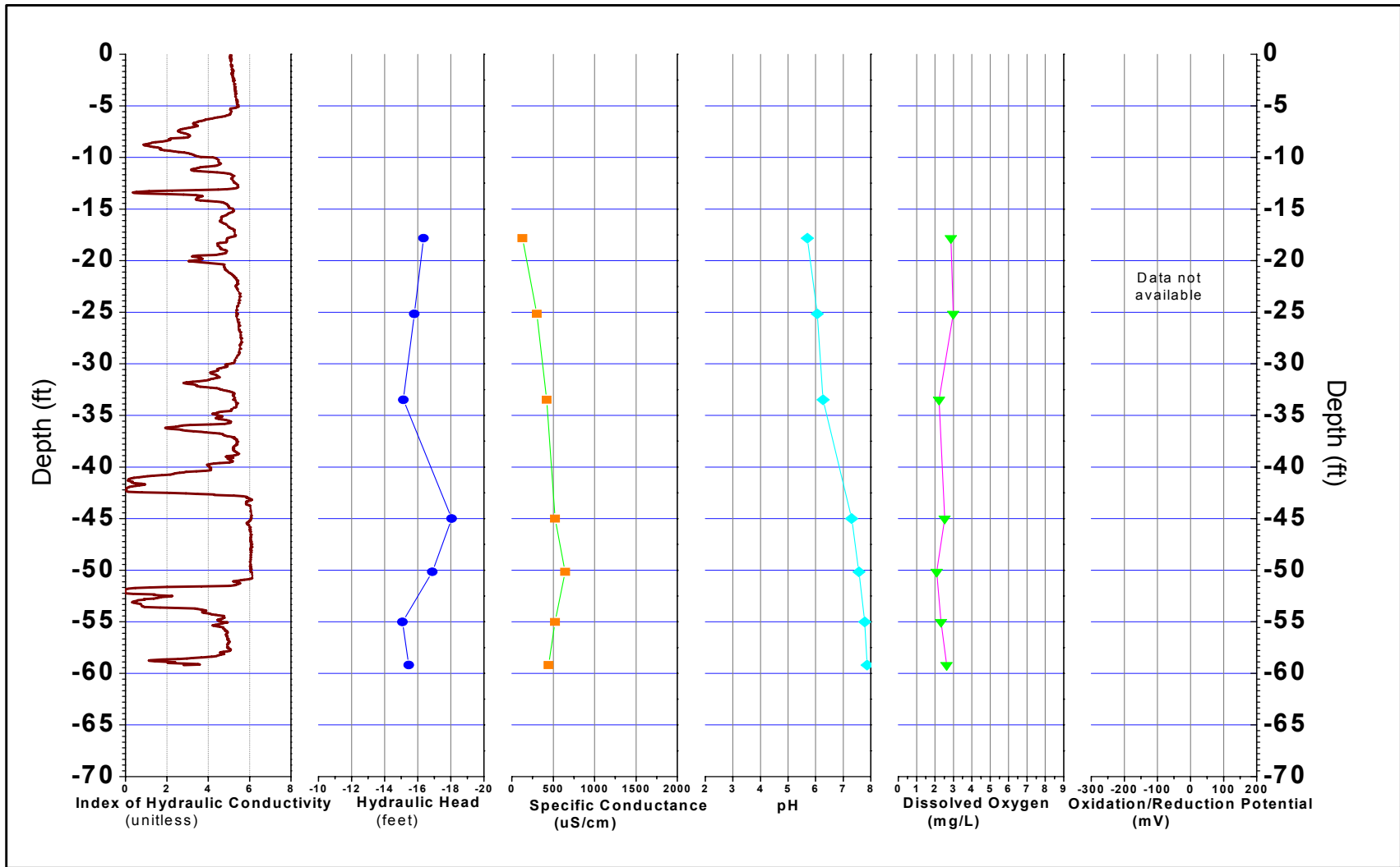
FIGURE B-233, I k RECORD AND PHYSICO-CHEMICAL PARAMETERS ERM, Wayland, Massachusetts
