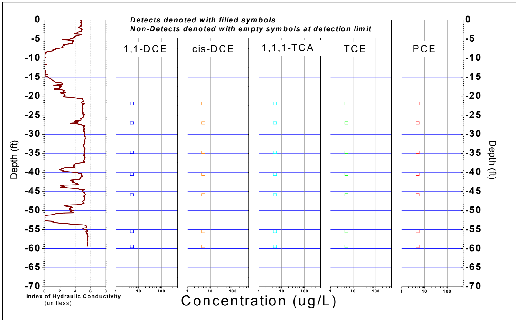
FIGURE B-235, I k RECORD AND SELECTED VOC ANALYTICAL RESULTS ERM, Wayland, Massachusetts
