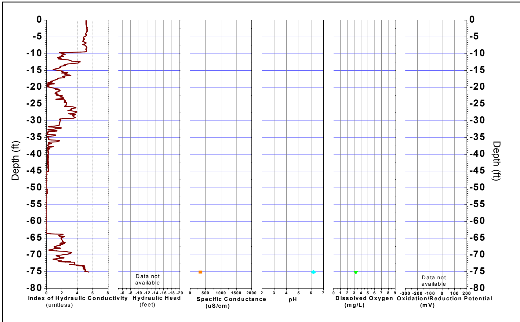
FIGURE B-232, I K RECORD AND PHYSICO-CHEMICAL PARAMETERS ERM, Wayland, Massachusetts
