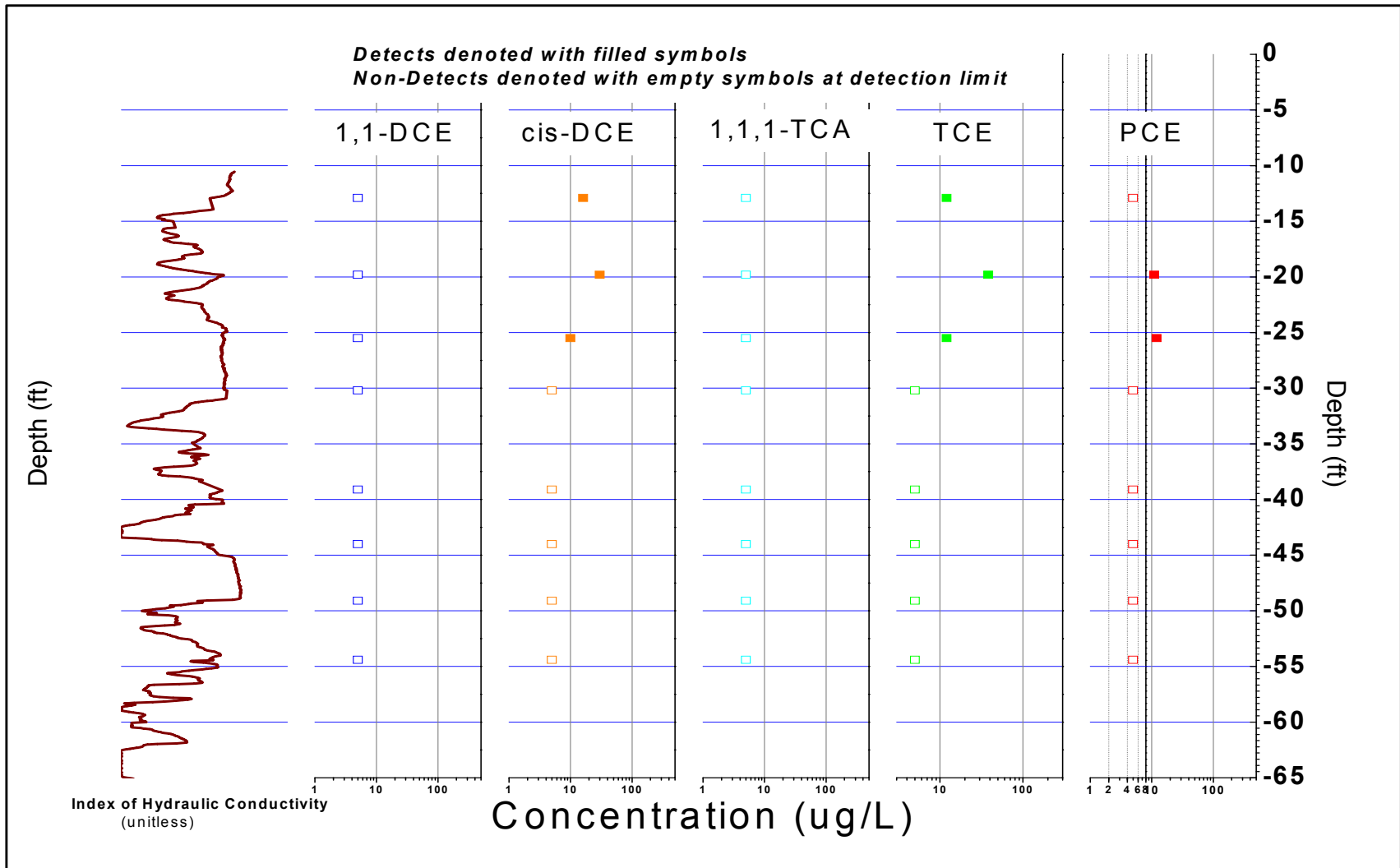
FIGURE B-221, I_k RECORD AND SELECTED VOC ANALYTICAL RESULTS ERM, Wayland, Massachusetts
