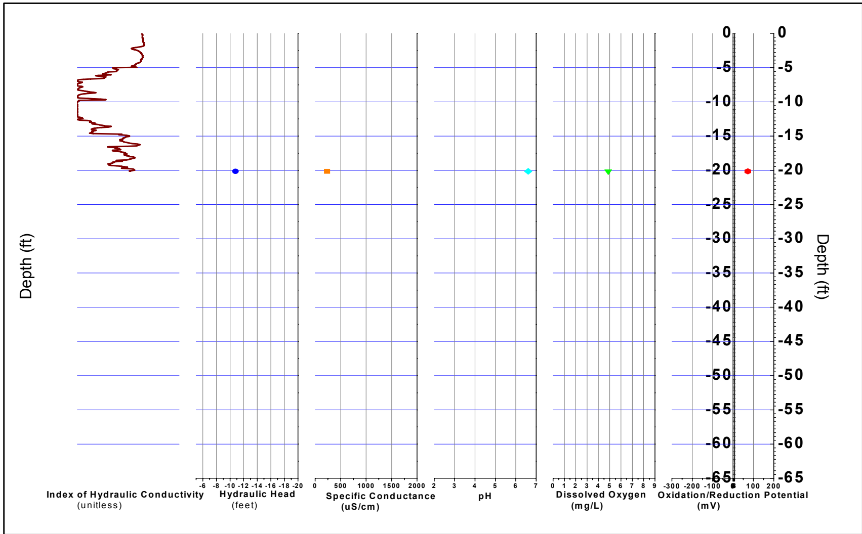
FIGURE B-242, I_k RECORD AND PHYSICO-CHEMICAL PARAMETERS ERM, Wayland, Massachusetts
